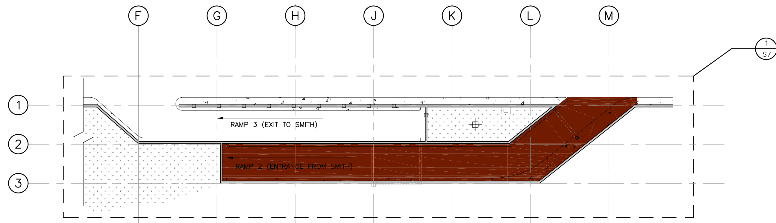
SMITH STREET LEVEL RAMP PLAN SCALE: 1/20"=1'-0"
