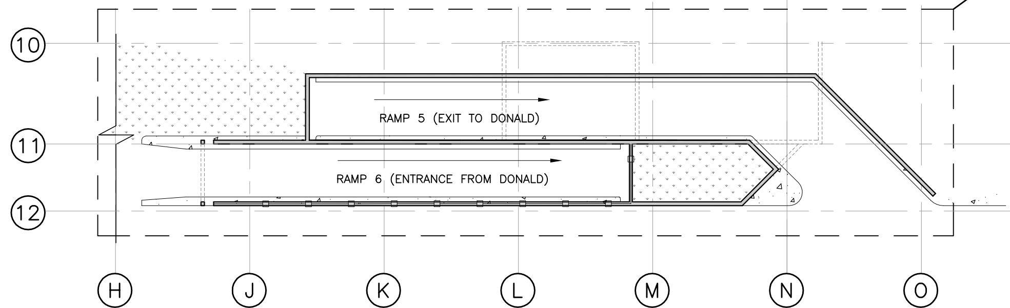
DONALD STREET LEVEL RAMP PLAN SCALE: 1/20"=1'-0"
