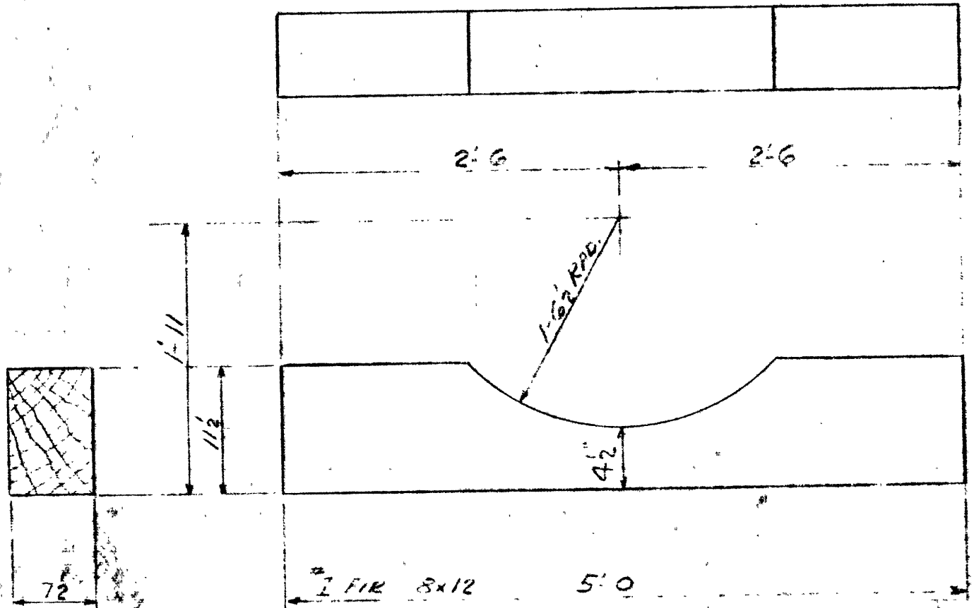
PIPE SADDLES - MARK SI - 15 REQ d (FOR 36" O.D. PIPE)
