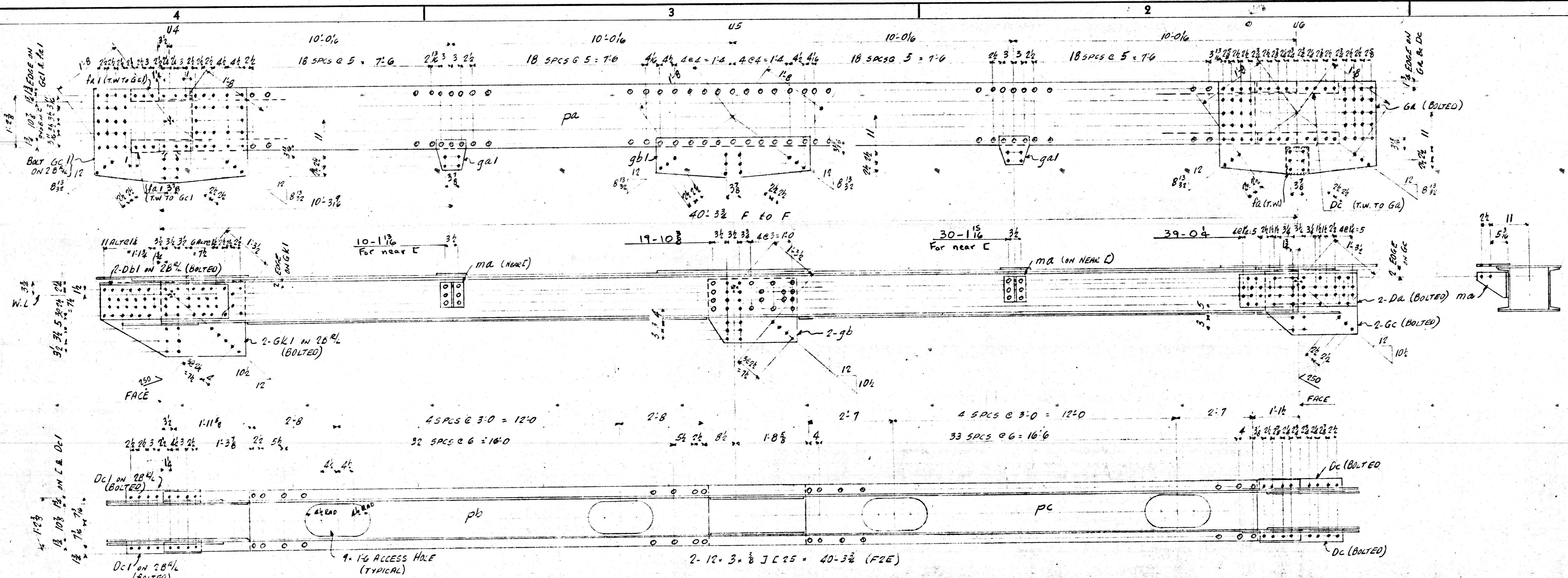
ONE-TOP CHORD SECTION 2A R ONE-TOP CHORD SECTION 2B R ONE- 10 2A L (LEFT) ONE- do 2B L (LEFT)
