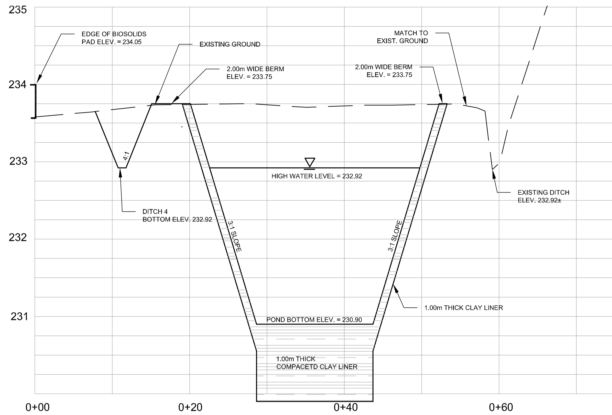
A BIOSOLIDS POND SECTION C-206 H: 1:250 V: 1:25
