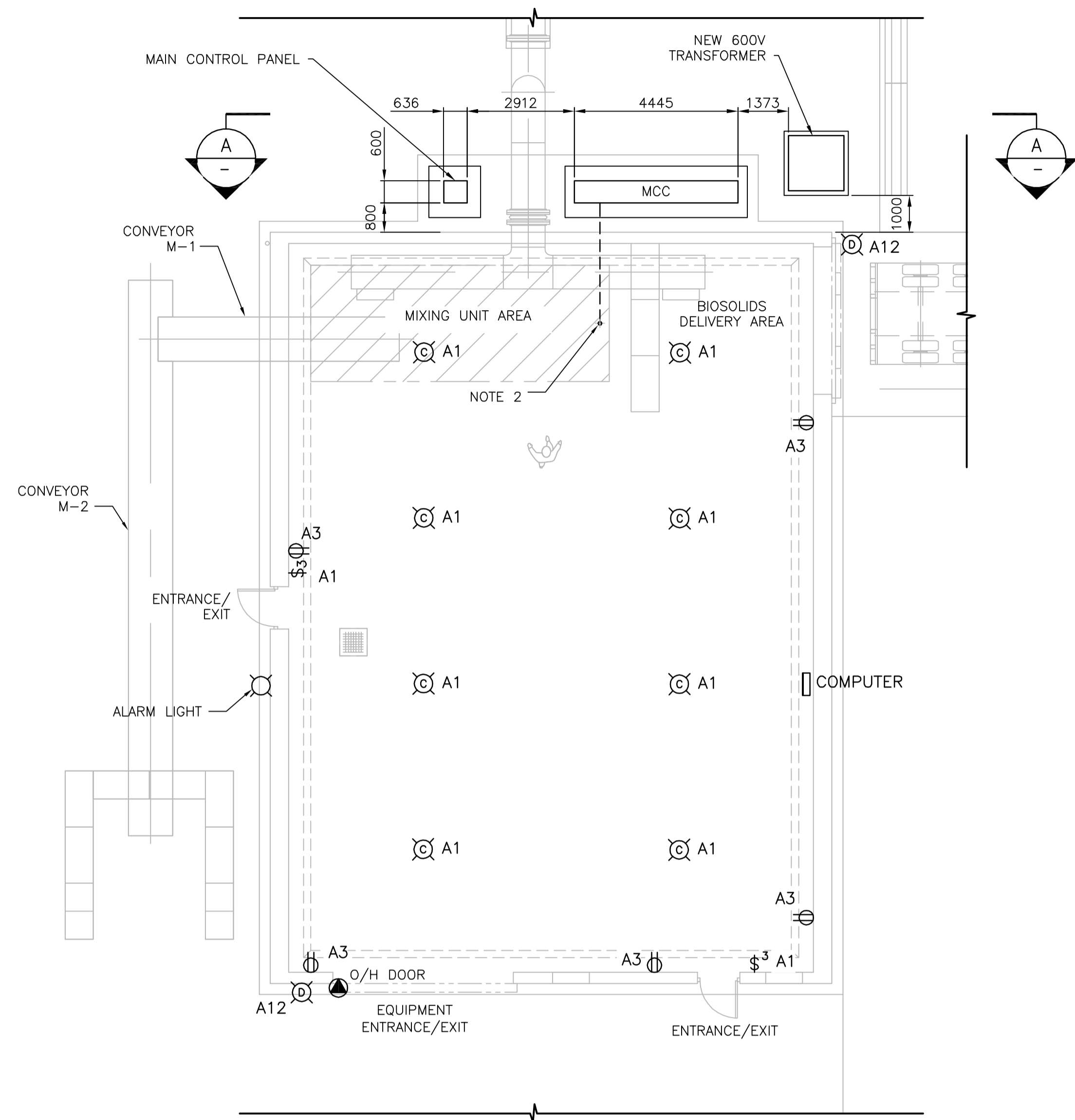
1 M&R BUILDING PLAN 1:100
