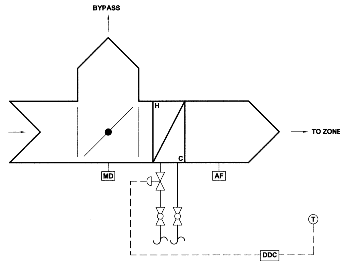
2 VAV (BYPASS BOX/HEATING COIL) (TYP.) Scale N.T.S.
