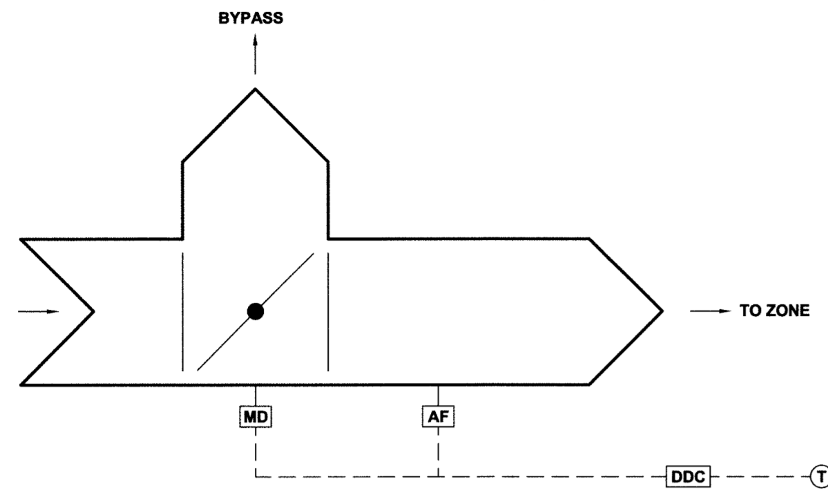
1 VAV (BYPASS) BOX (TYP.) Scale N.T.S.
