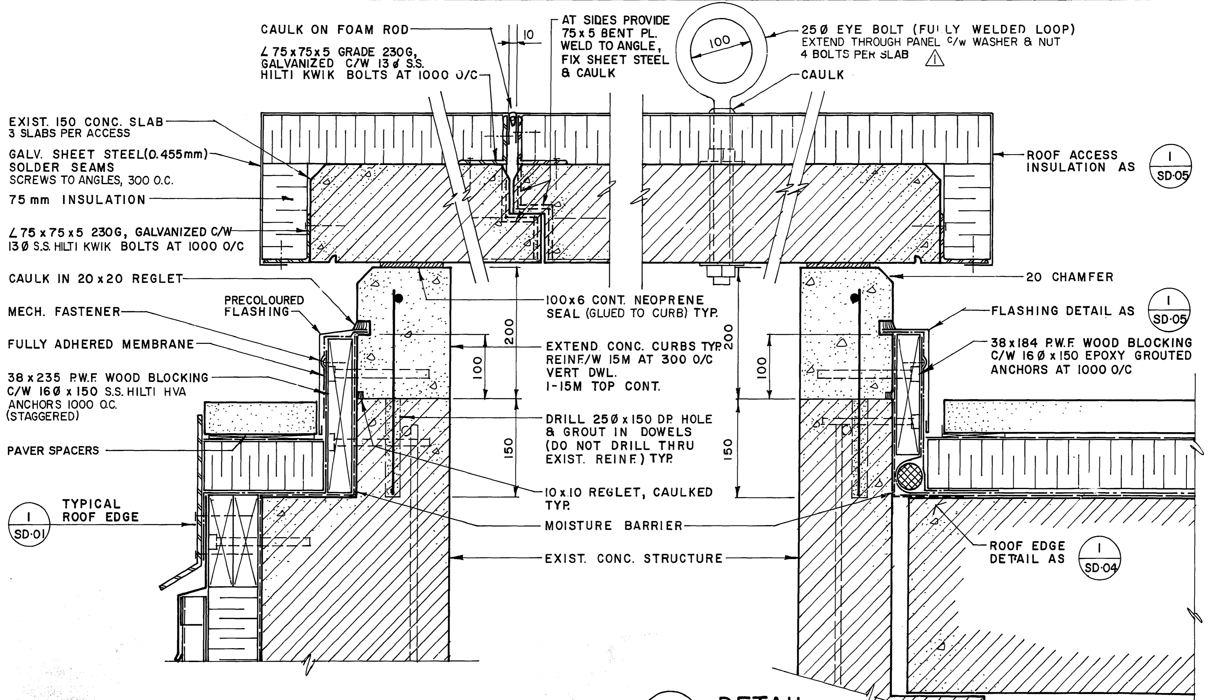
1 SD-05 DETAIL 1:5
