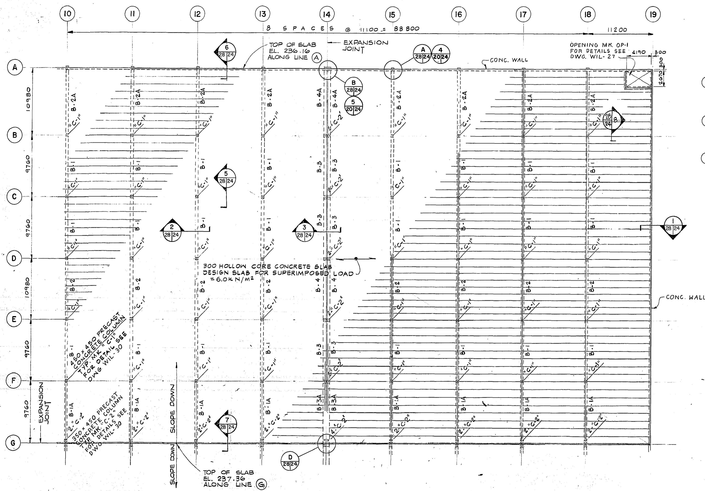
ROOF PLAN AREA B
