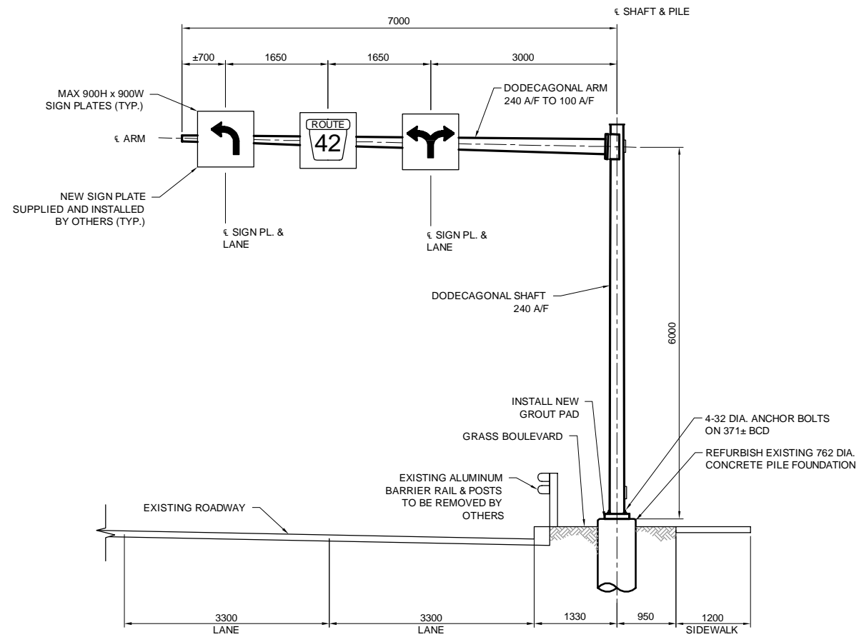
SITE ELEVATION - LOOKING WEST OVERHEAD SIGN SUPPORT STRUCTURE NO. S622
