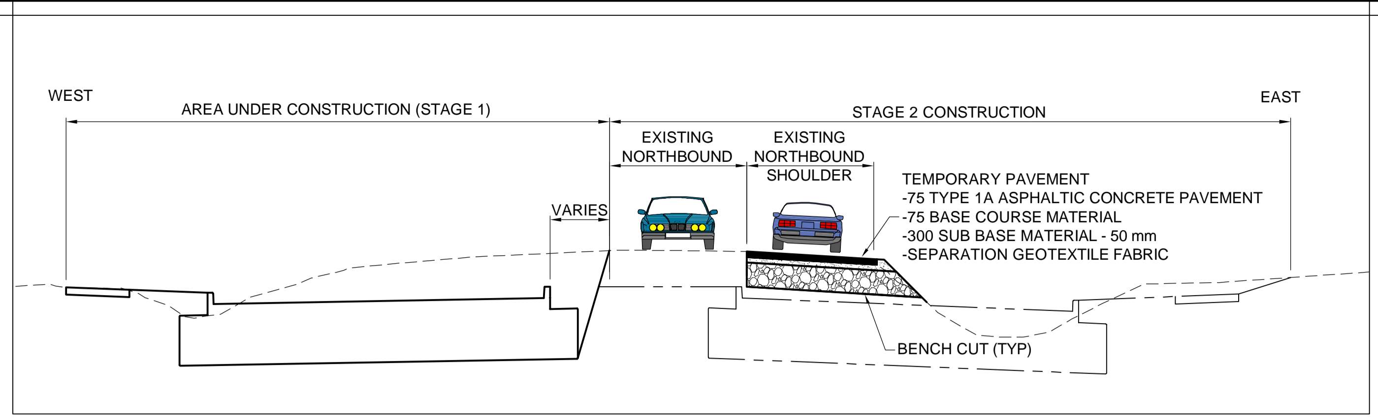
TYPICAL STAGE 1 SECTION
