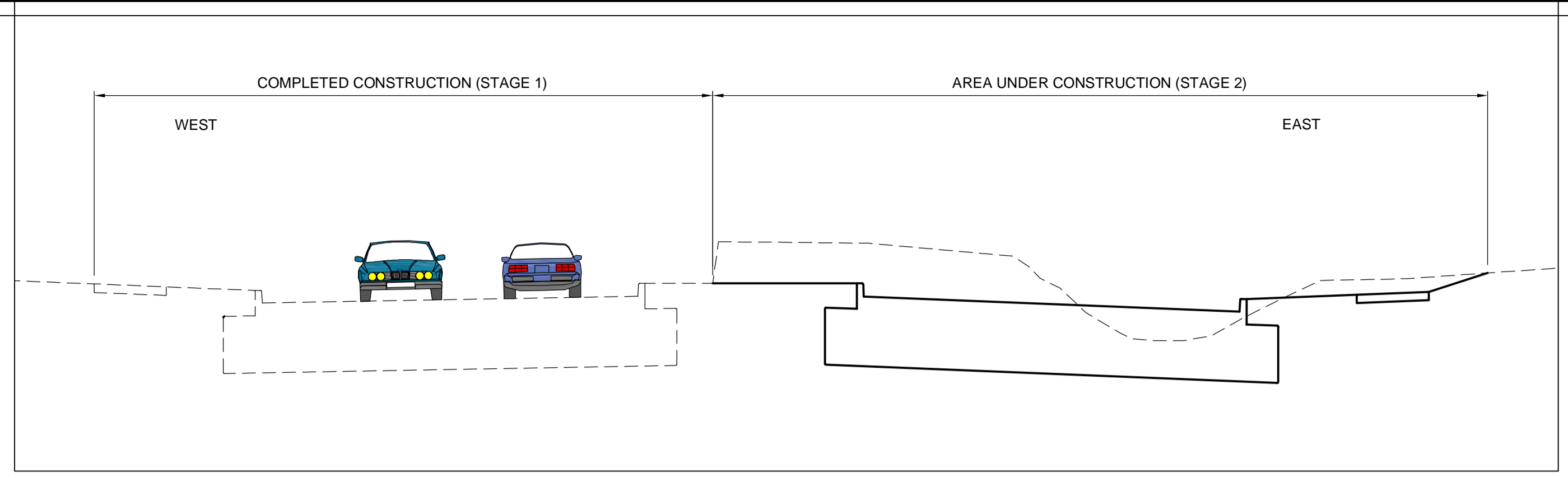
TYPICAL STAGE 2 SECTION
