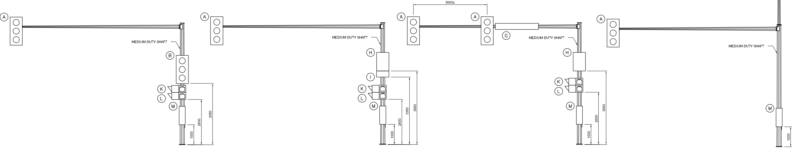
M26-Da TYPE D-T BREAKAWAY BASE
