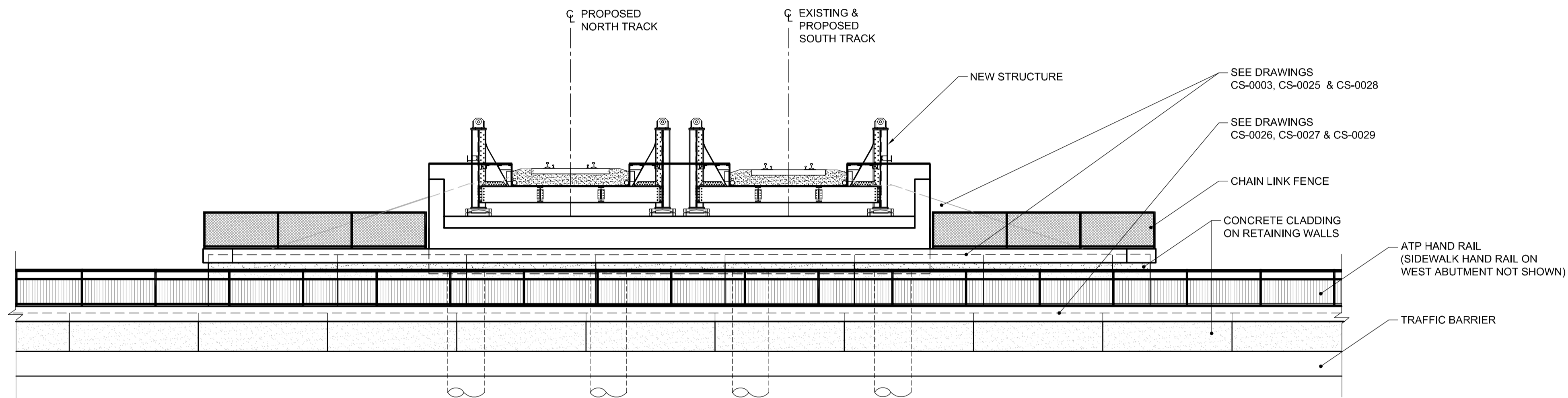
A SECTION - EAST ABUTMENT (PHASE VI, STAGE 2) CS-0004 Scale 1:100 (WEST ABUTMENT SIMILAR)
