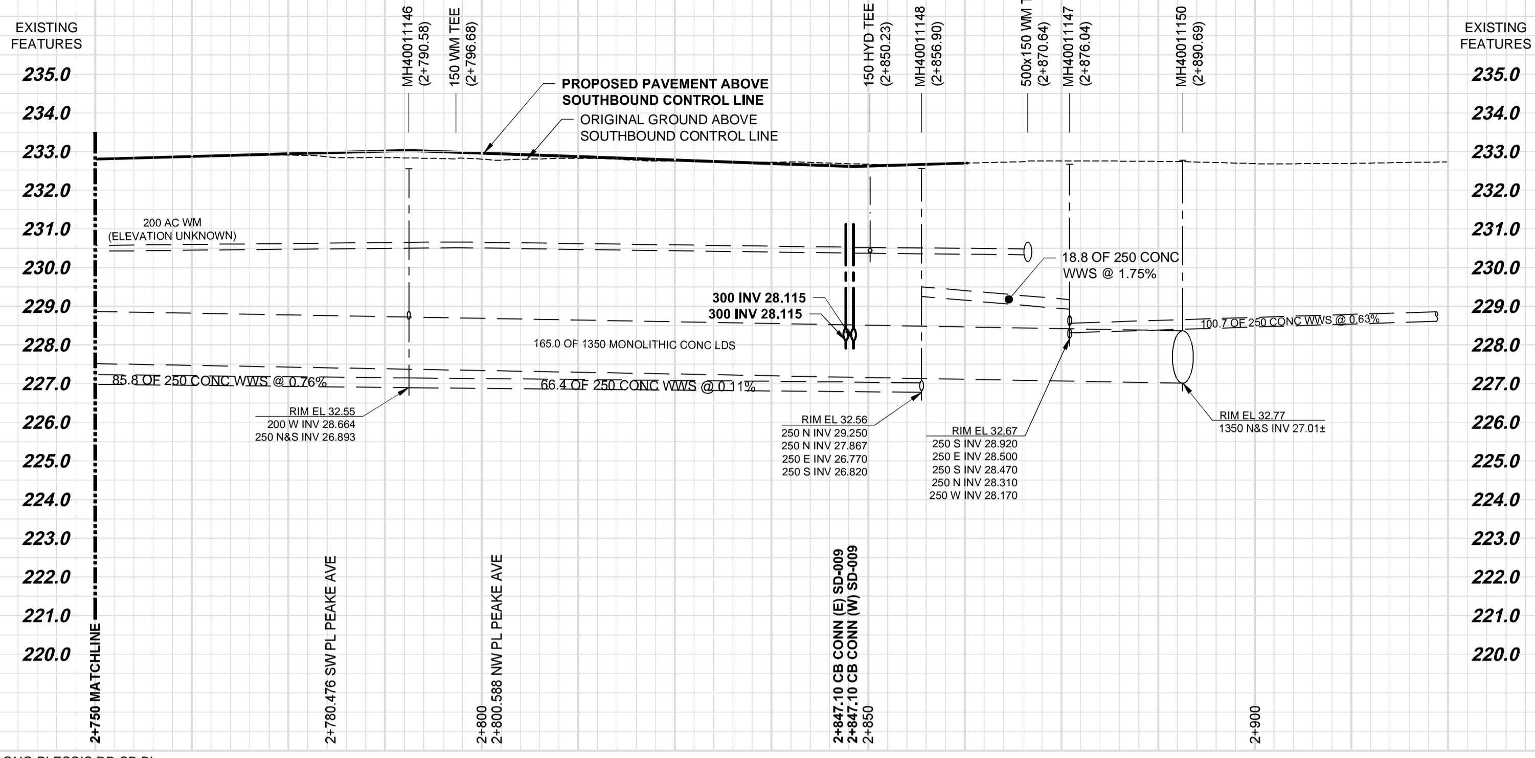
CHAINAGE ALONG PLESSIS RD SB BL
