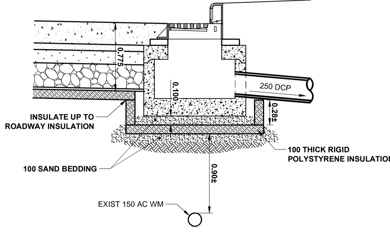
CATCHPIT INSULATION DETAIL Scale 1:25
