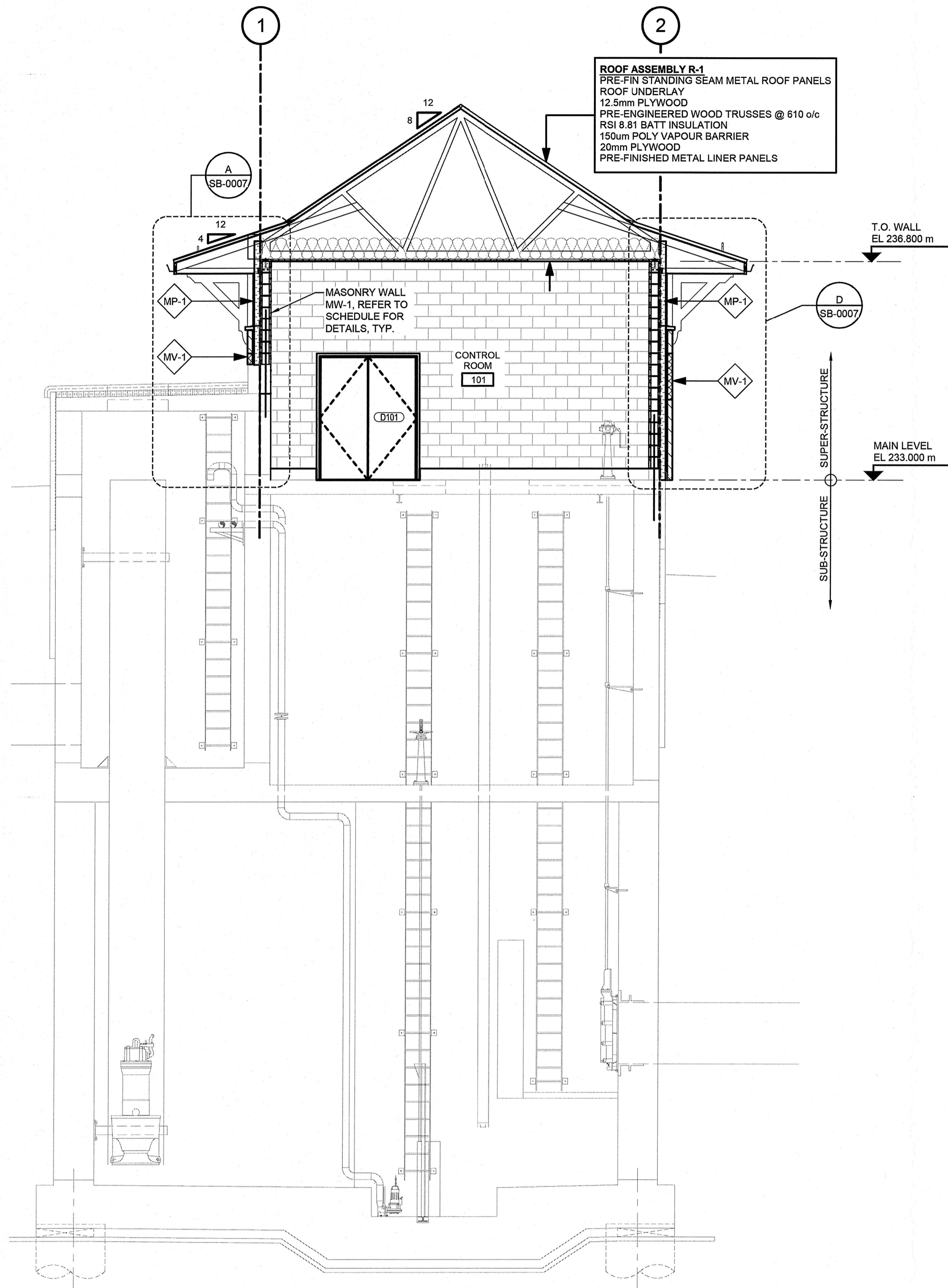
A SECTION A SB-0003 1:50
