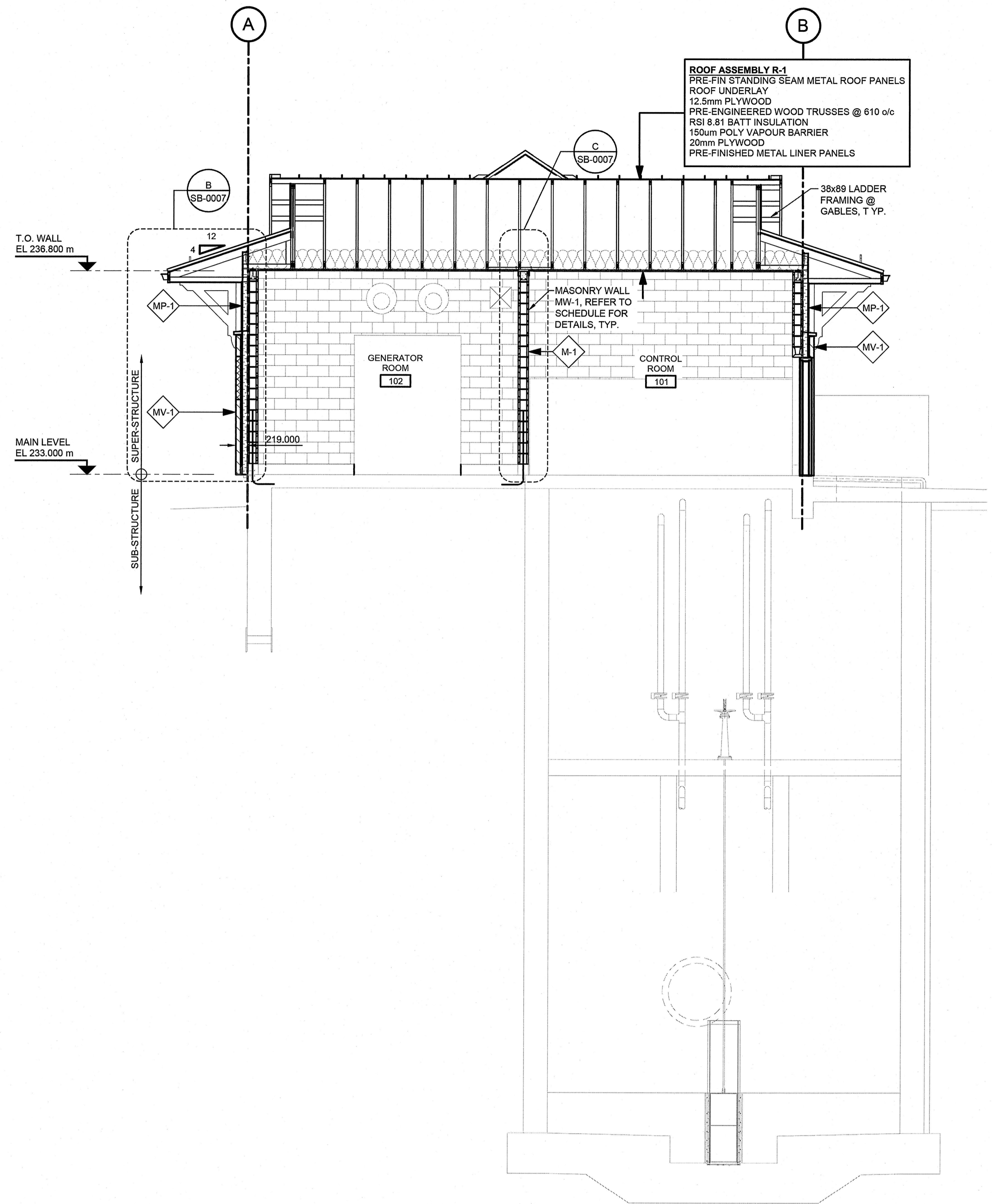
B SECTION B SB-0003 1:50
