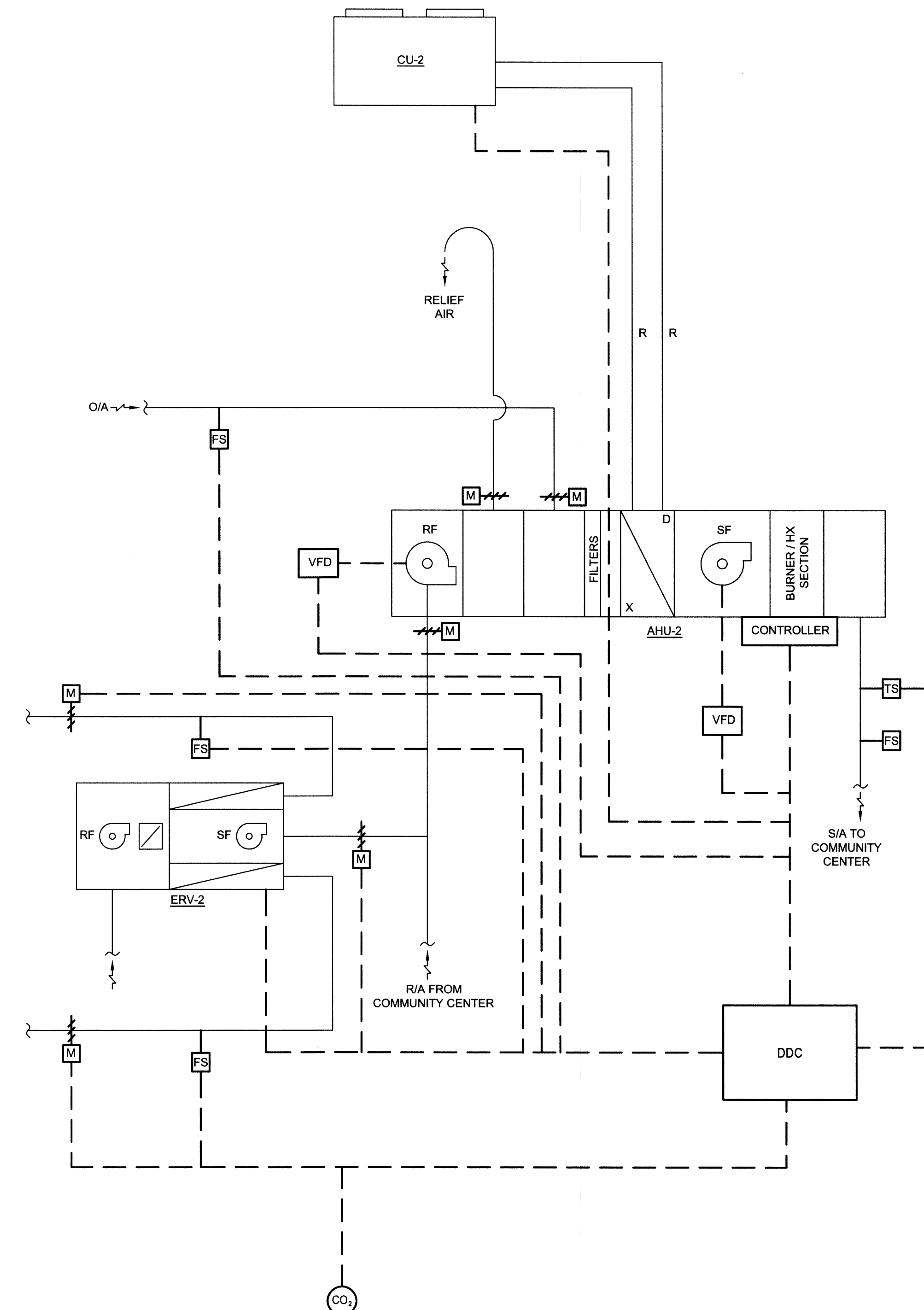
NOTE: CO 2 SENSORS LOCATED IN THE OCCUPIED SPACE NOTE: VFD'S SUPPLIED AND INSTALLED BY CONTROLS CONTRACTOR. REFER TO ELECTRICAL FOR SPECIFICATIONS. 2 AHU-2 CONTROL SCHEMATIC SCALE: N.T.S.
