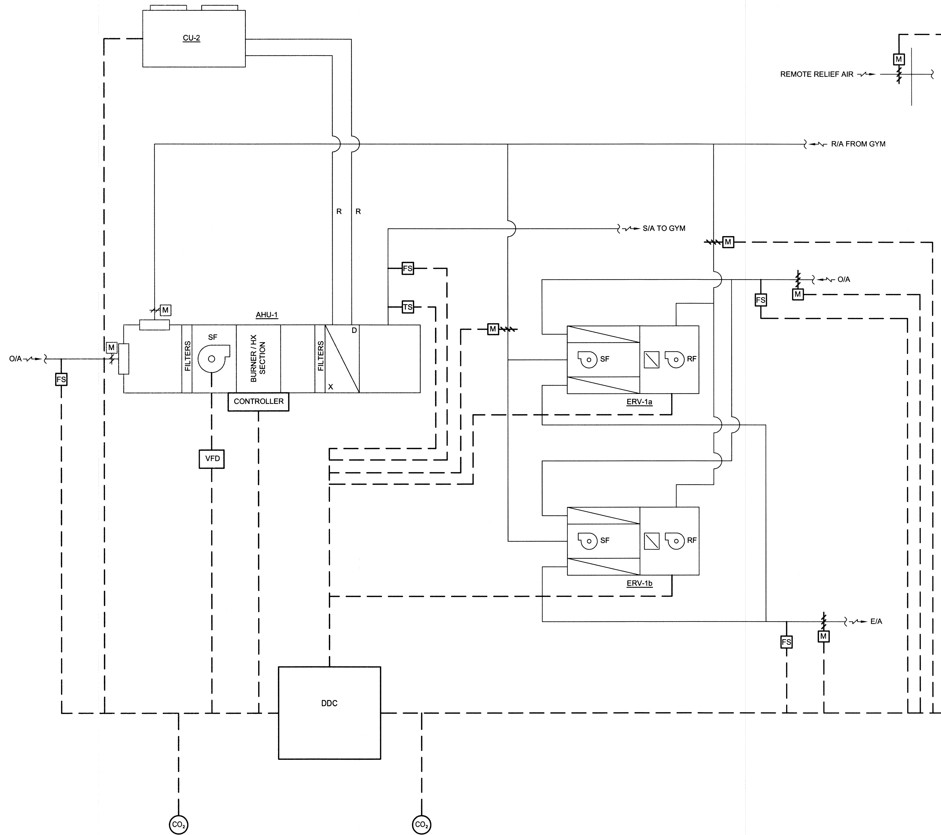
NOTE: CO 2 SENSORS LOCATED IN THE OCCUPIED SPACE NOTE: VFD'S SUPPLIED AND INSTALLED BY CONTROLS CONTRACTOR. REFER TO ELECTRICAL FOR SPECIFICATIONS. 1 AHU-1 CONTROL SCHEMATIC SCALE: N.T.S.
