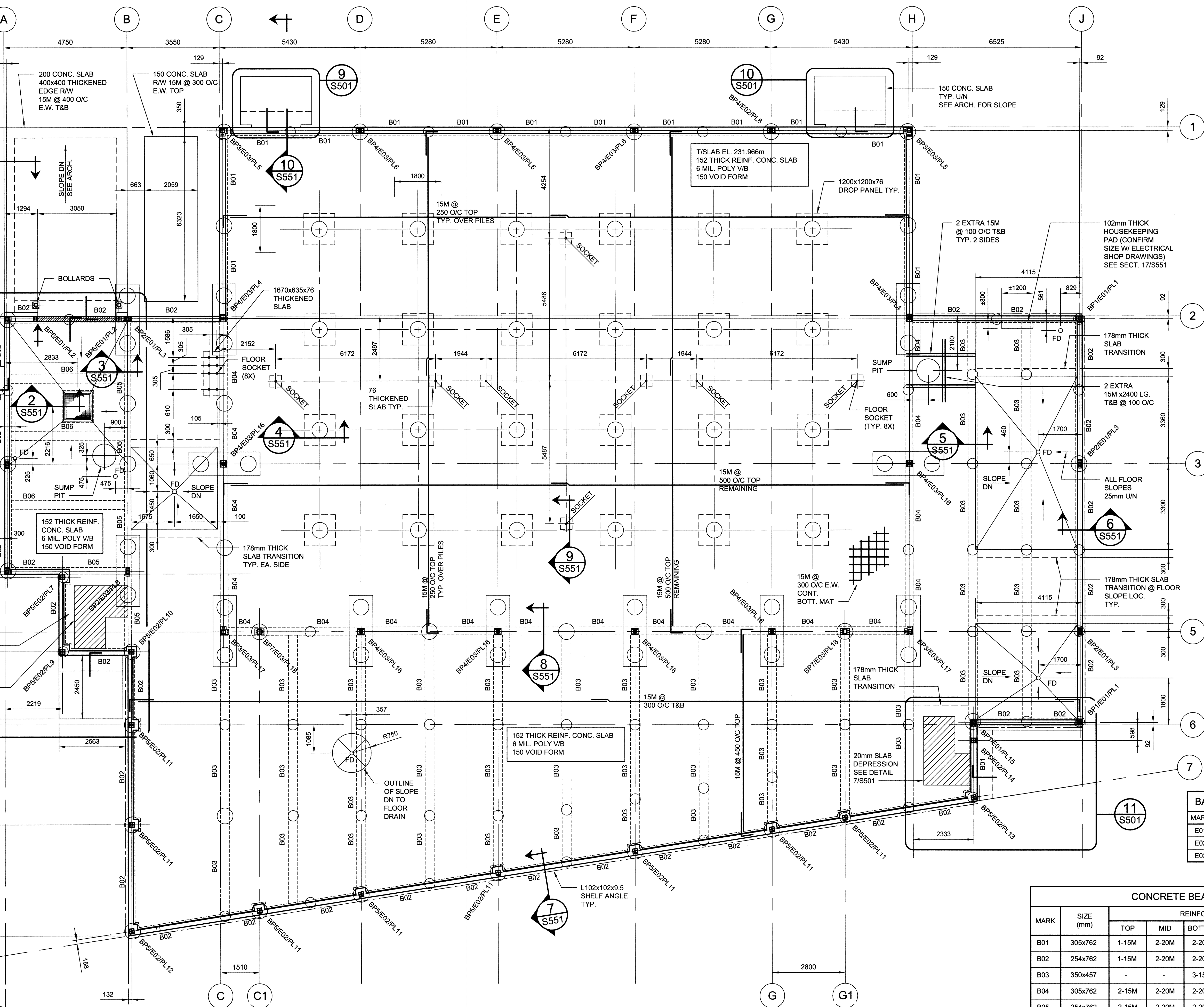
1 MAIN FLOOR FRAMING PLAN 1:76
