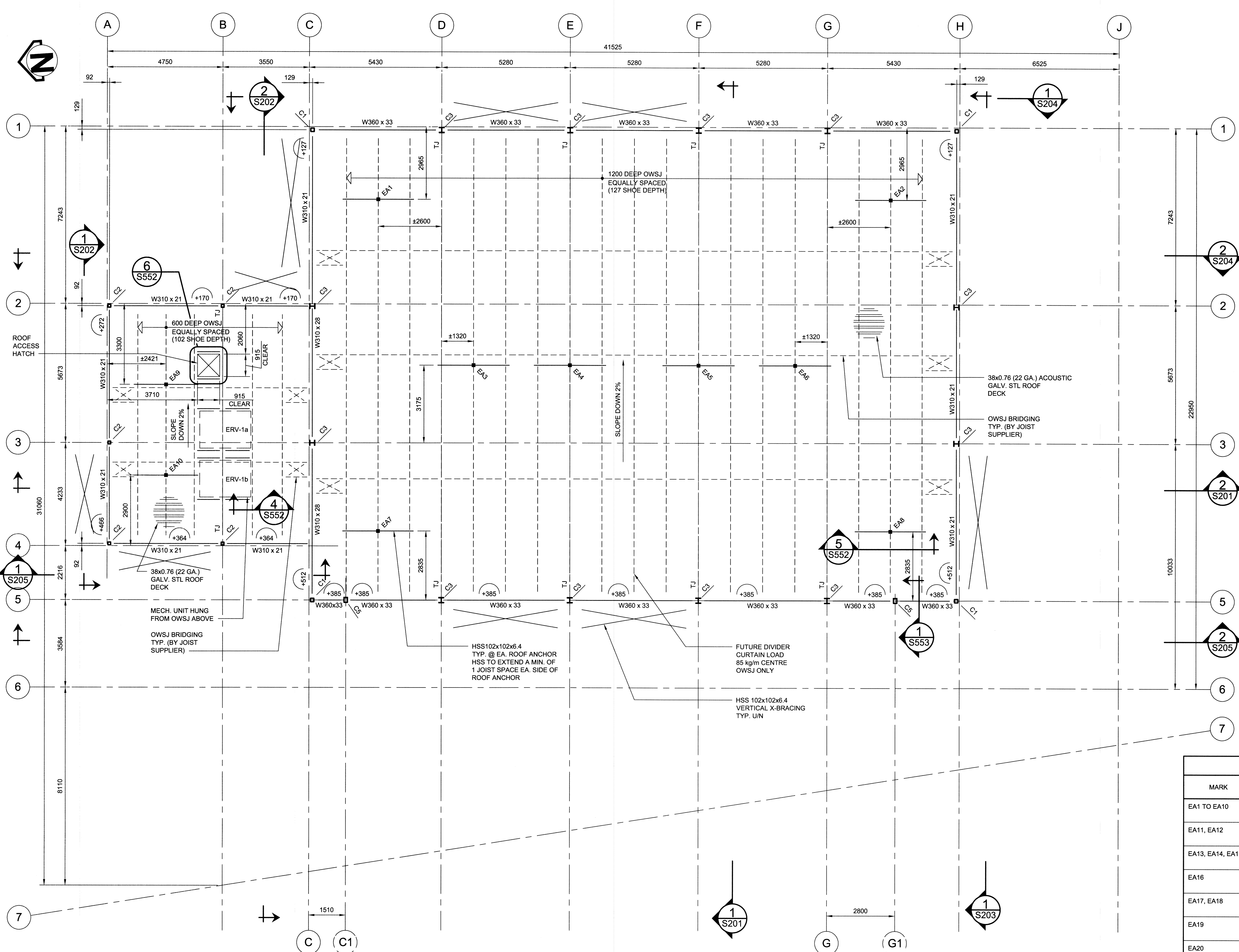
1 HIGH ROOF FRAMING PLAN 1:75 T/STEEL EL. 109.023m U/N
