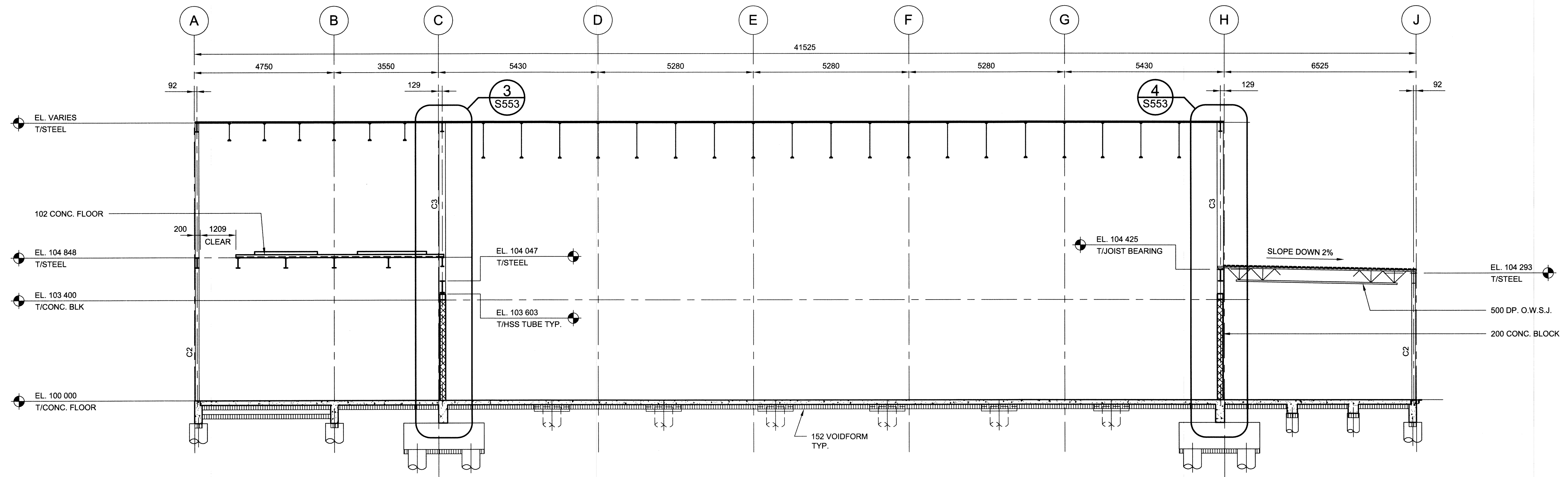
2 SECTION @ GRIDLINE '3' - LOOKING EAST 1:75
