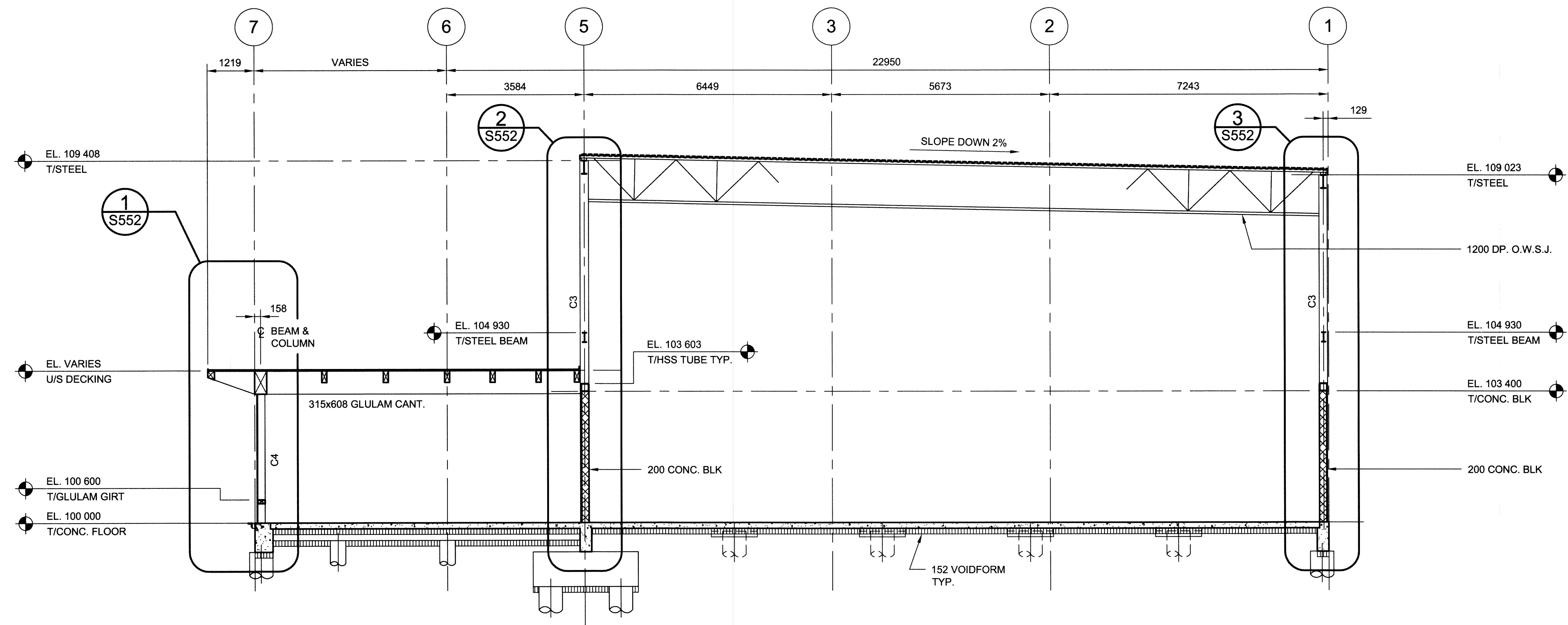
1 SECTION @ GRIDLINE 'F' - LOOKING NORTH 1:75
