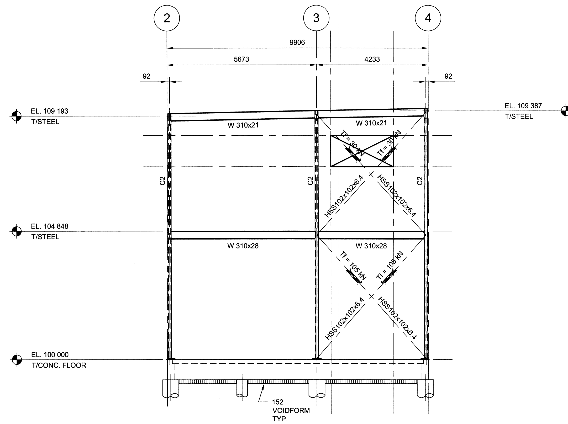
1 GRIDLINE 'A' ELEVATION - LOOKING SOUTH 1:75
