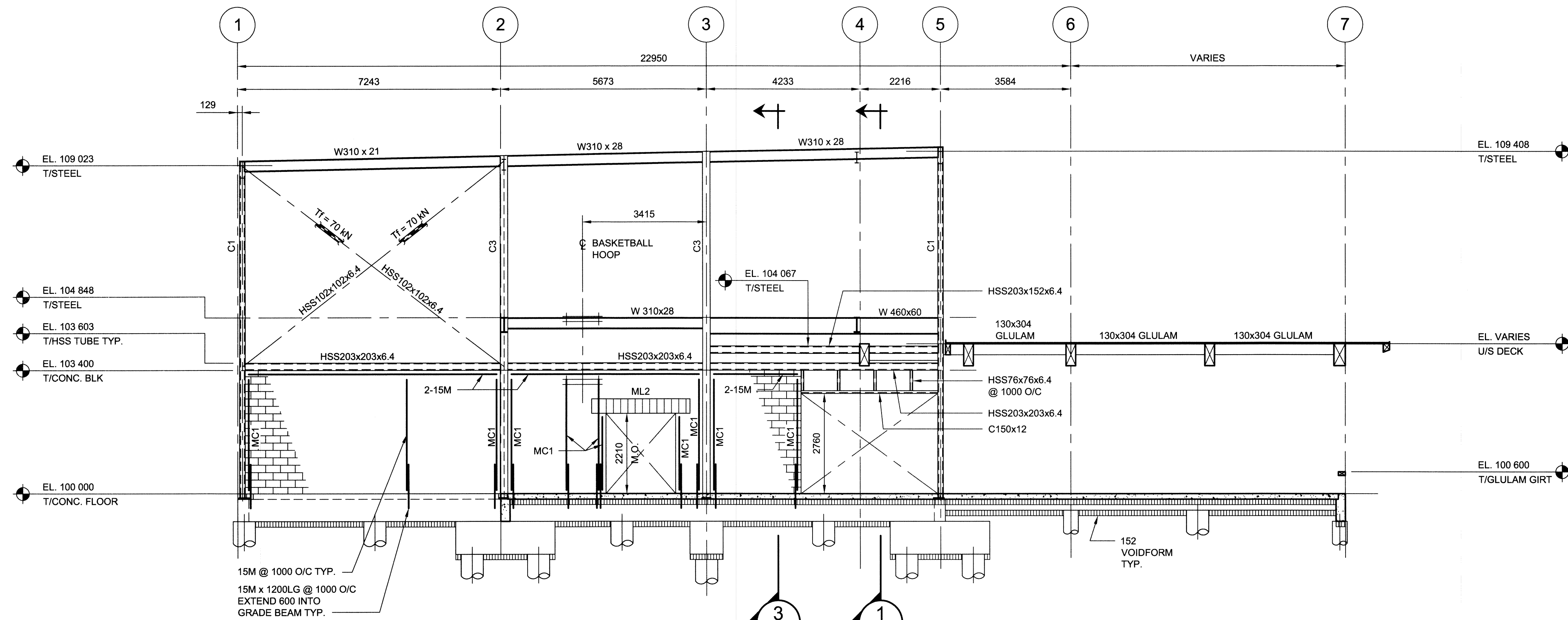
2 GRIDLINE 'C' ELEVATION - LOOKING SOUTH 1:75
