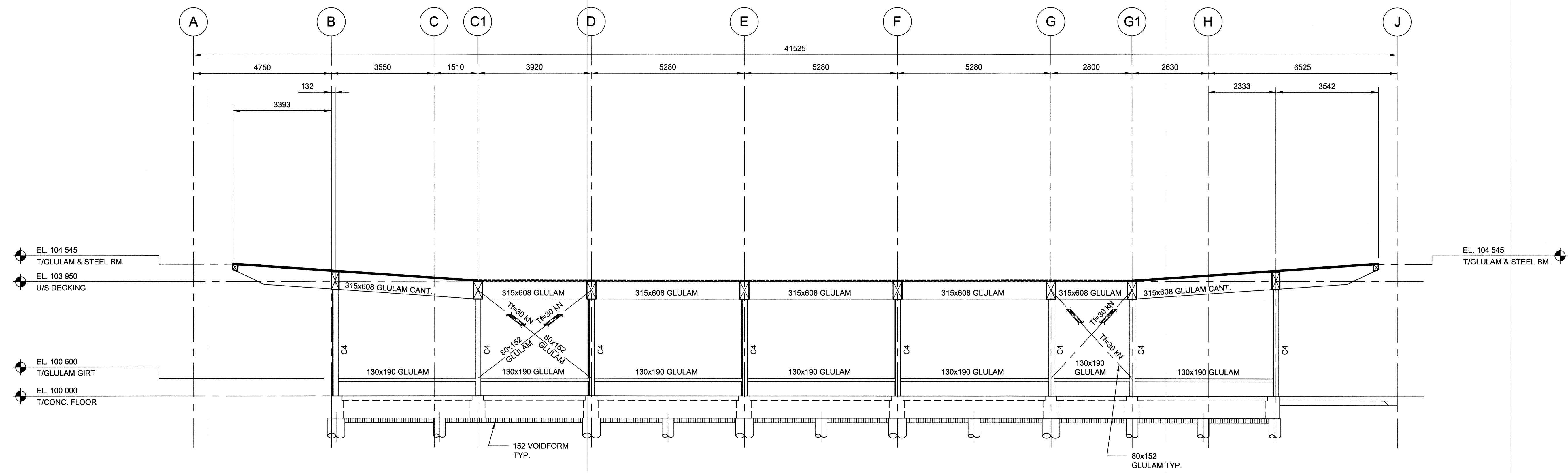
1 GRIDLINE '7' ELEVATION - LOOKING EAST 1:75
