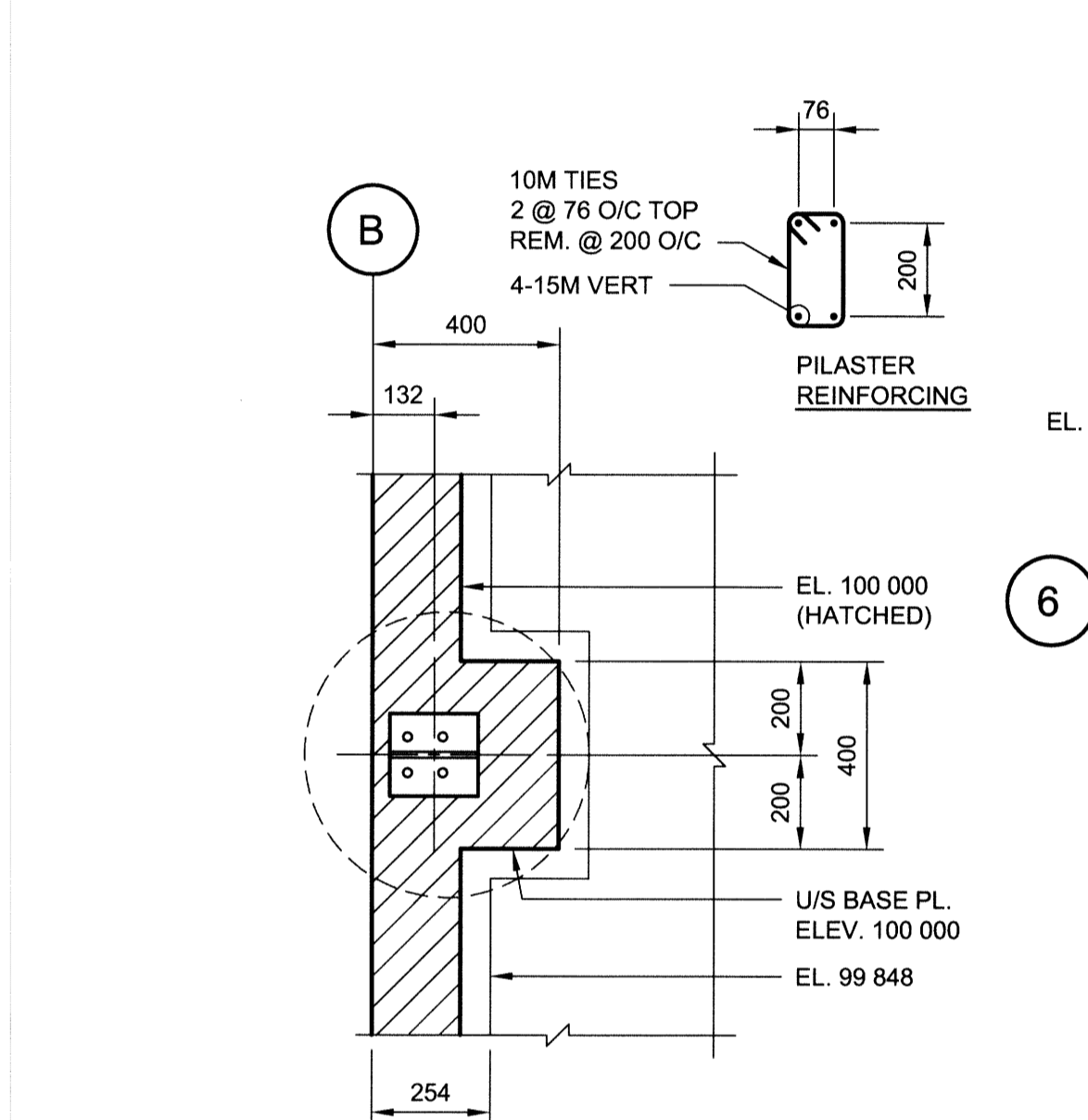
8 DETAIL - PL11 1:15
