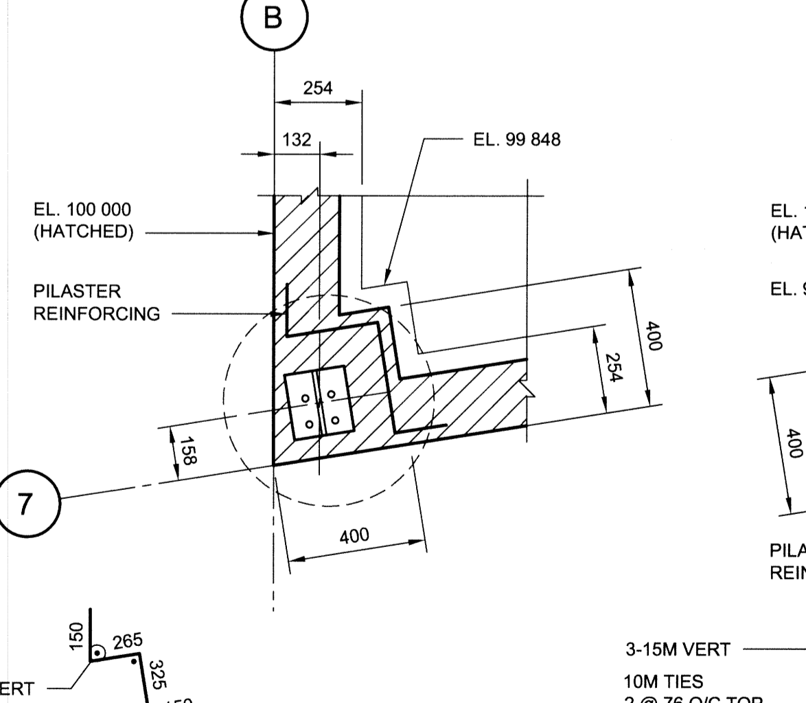
12 DETAIL - PL12 1:15
