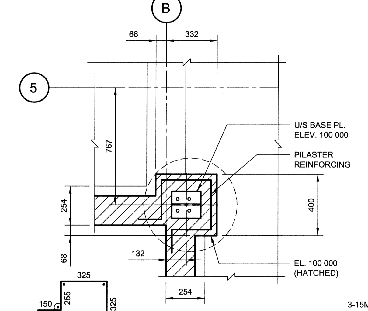
11 DETAIL - PL10 1:15
