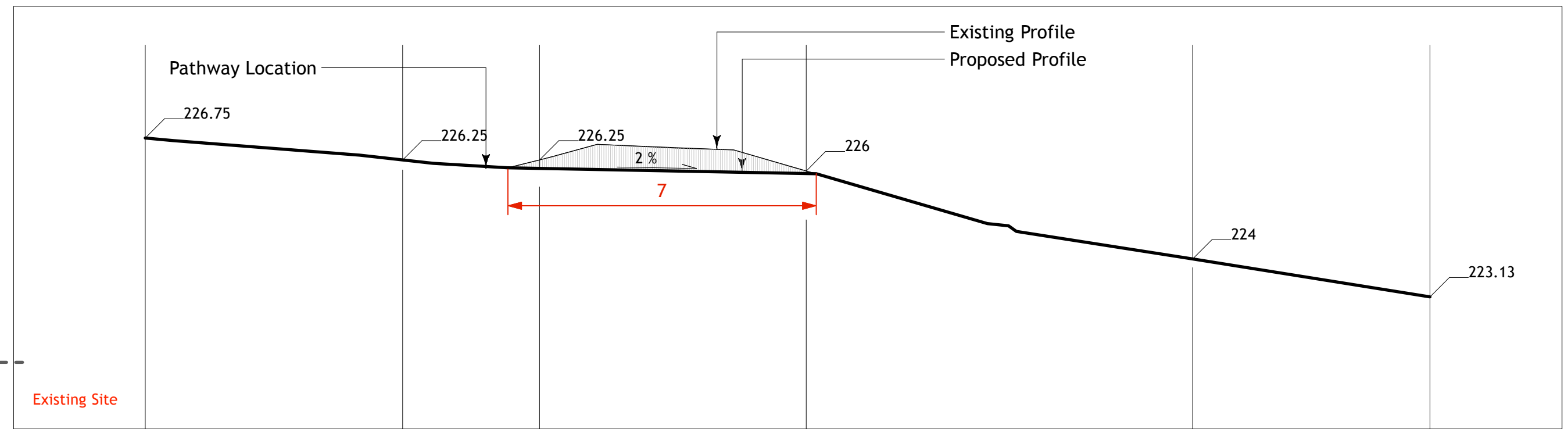
2 Typical Cross Section - Drain Outlet L-04 Scale: 1:100
