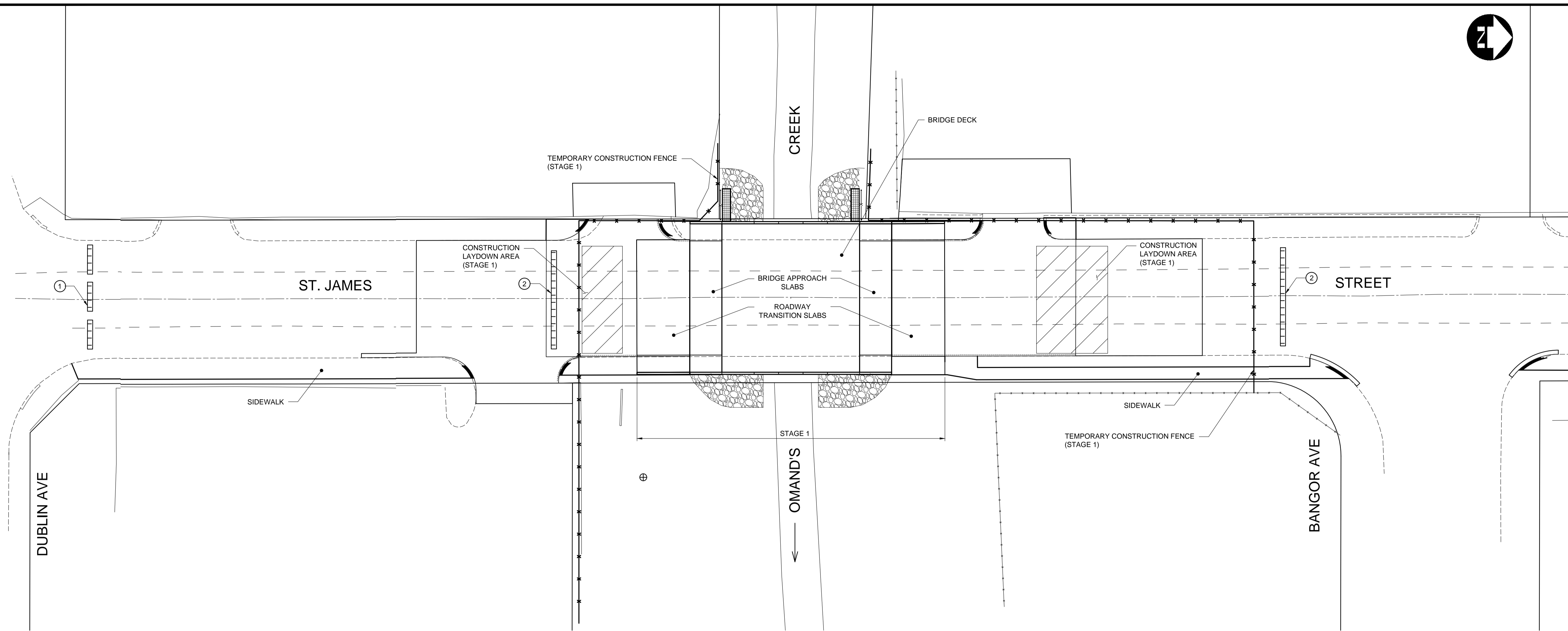
PLAN NTS
