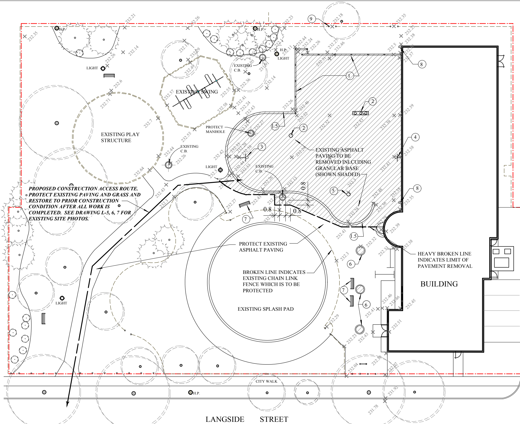
1 EXISTING SITE / DEMOLITION PLAN L1 Scale: 1:300
