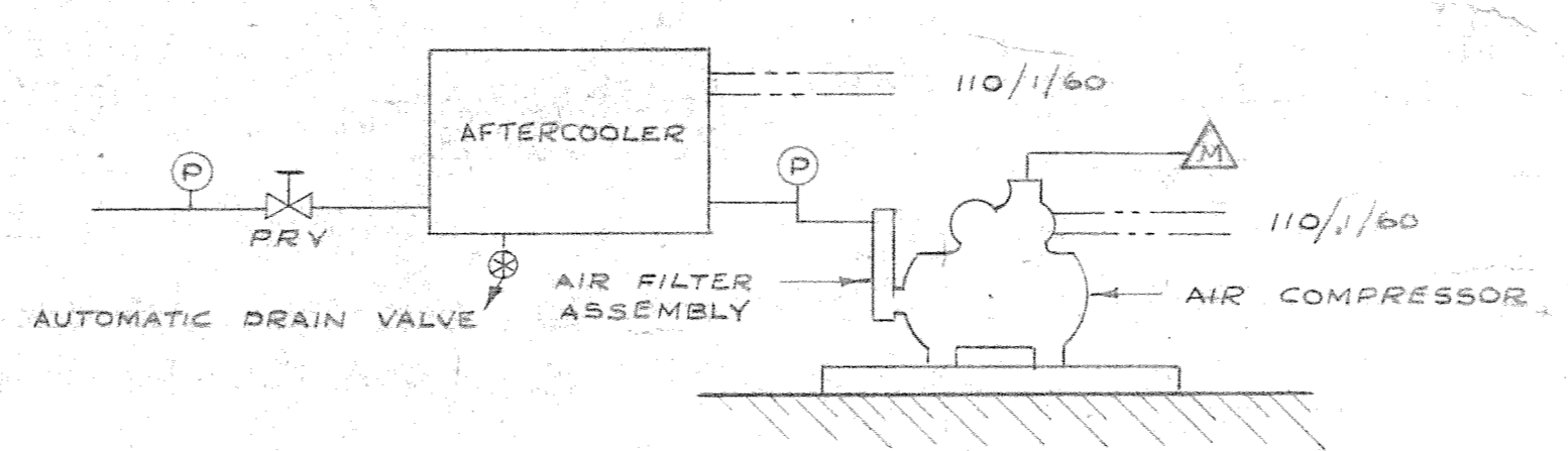
COMPRESSED AIR SUPPLY NOT TO SCALE
