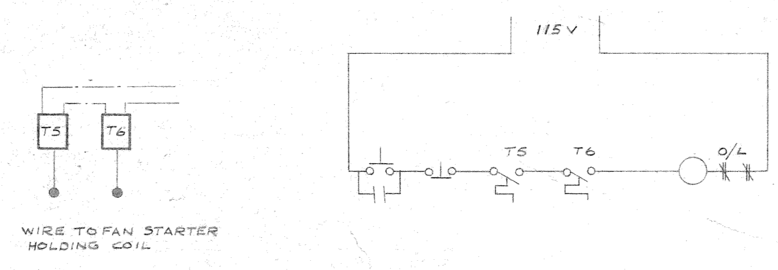
WIRING DIAGRAM FOR A/C SAFETY CONTROLS NOT TO SCALE
