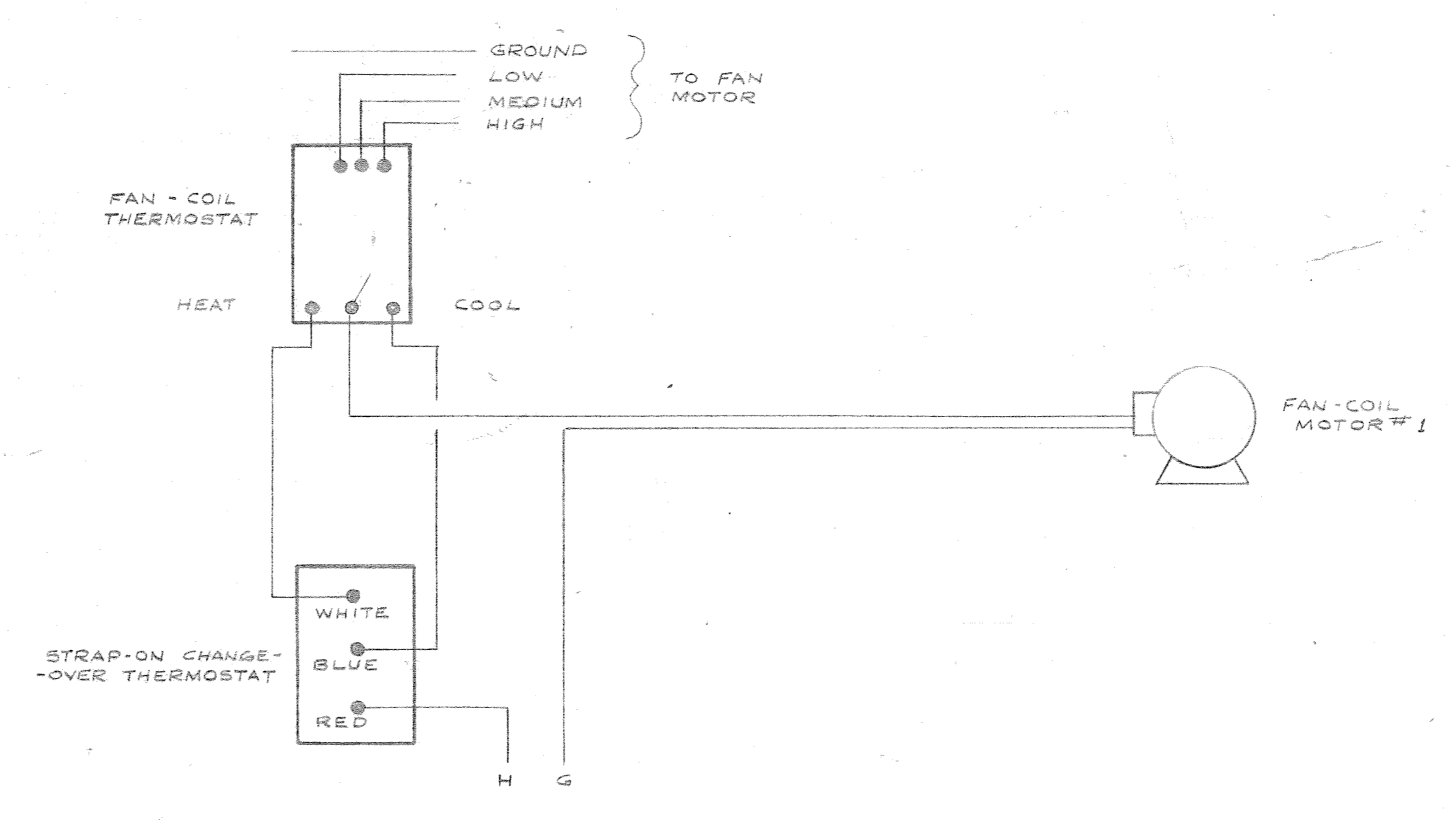
CONTROLS OF FAN-COIL UNITS NOT TO SCALE
