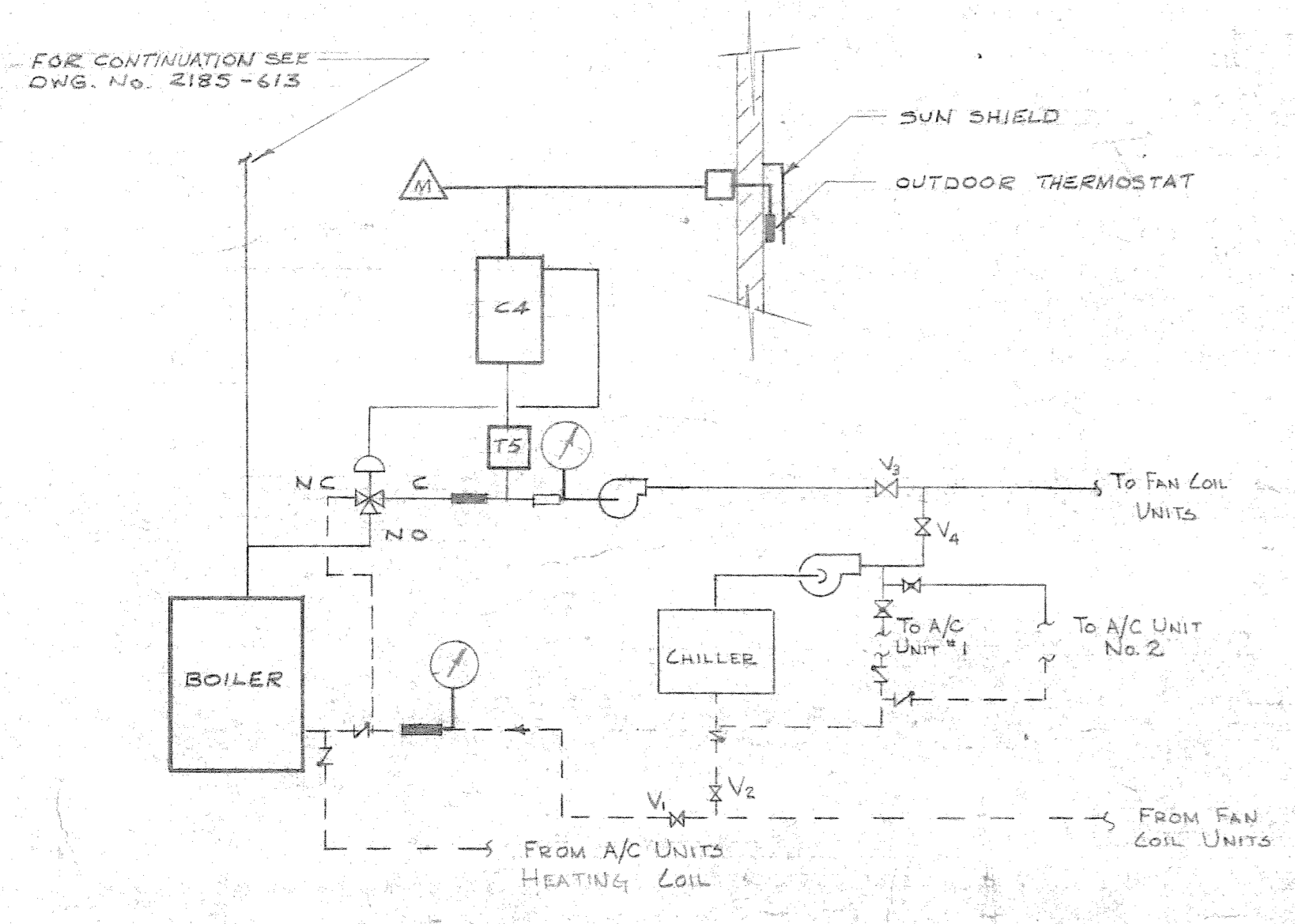
SCHEMATIC CONTROL DIAGRAM HOT & CHILLED WATER CIRCUITS NOT TO SCALE (AUTOMATIC RESET OF HOT WATER TEMPERATURE TO FAN-COIL UNITS FROM OUTDOOR TEMPERATURE)
