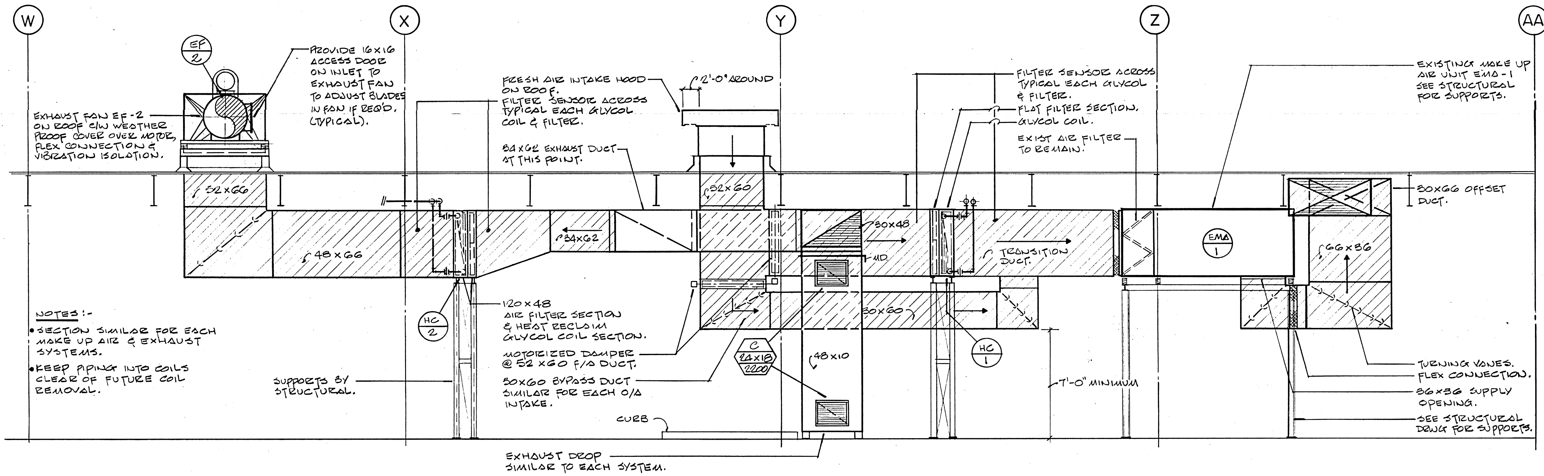
SECTION DETAIL 2/M2 SCALE: 1/4" = 1'-0"
