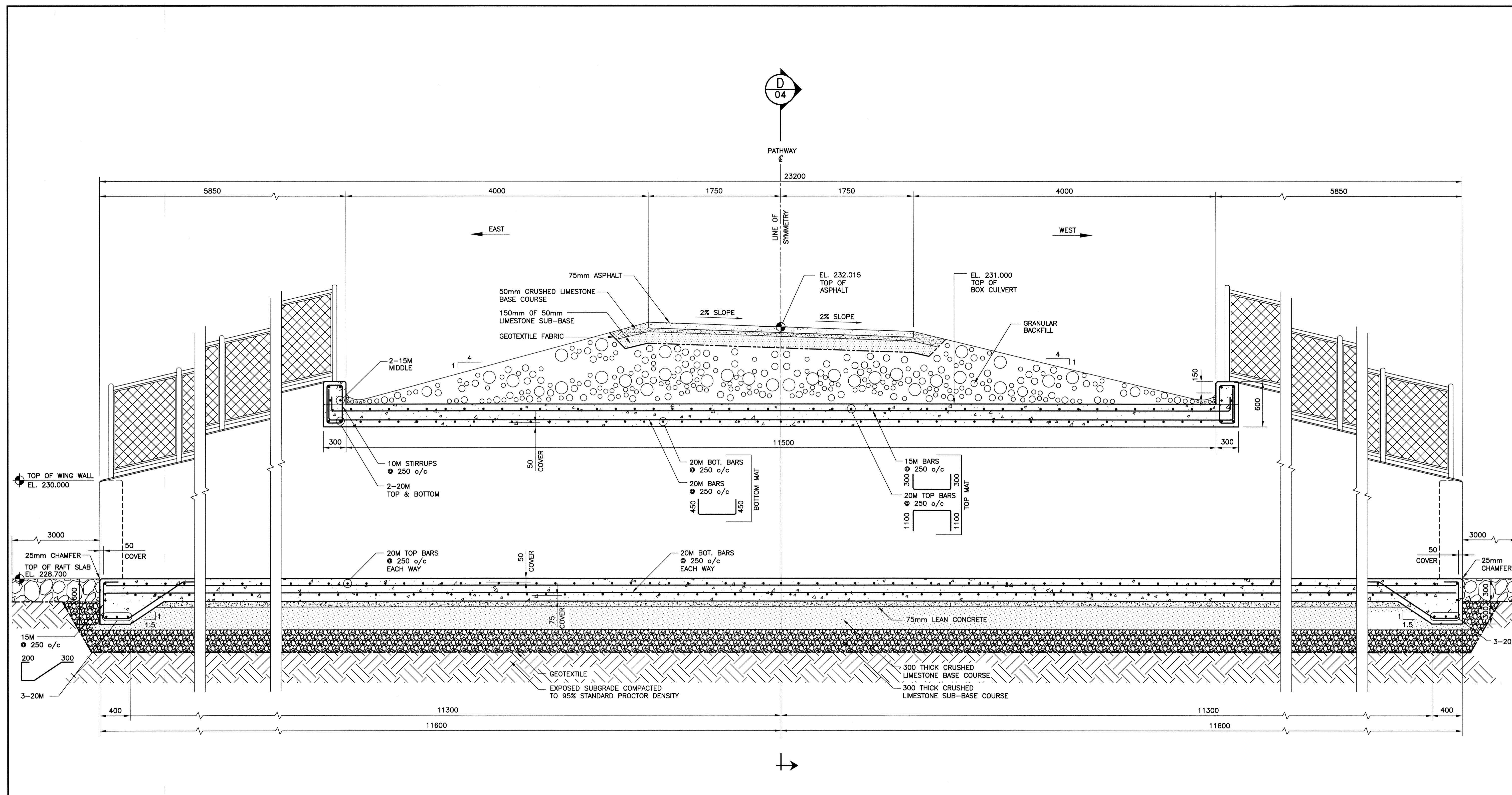
(C) BOX-CULVERT SECTION SCALE: 1:25 1:50
