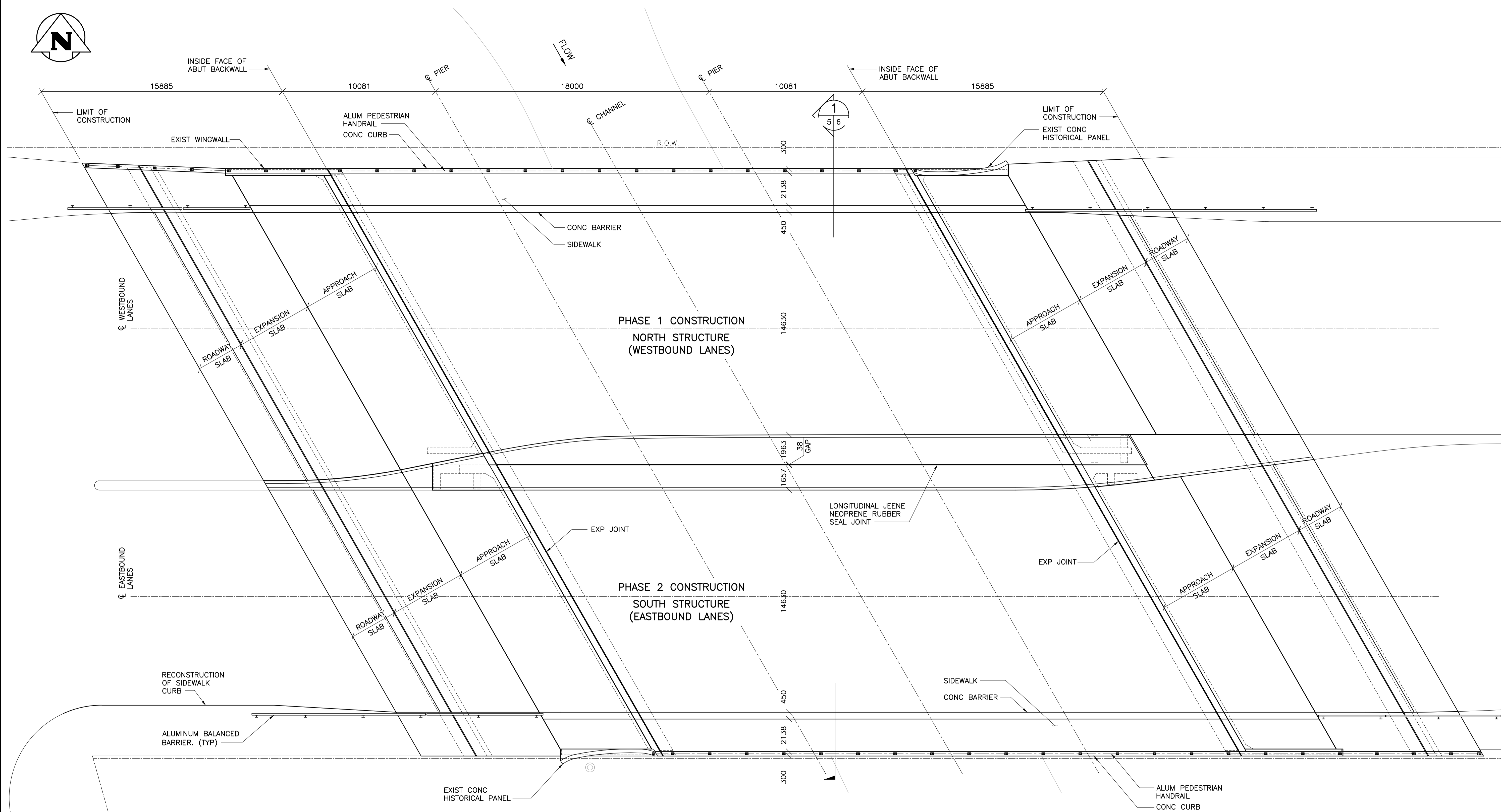
1 - - GENERAL ARRANGEMENT - PLAN 1 : 125
