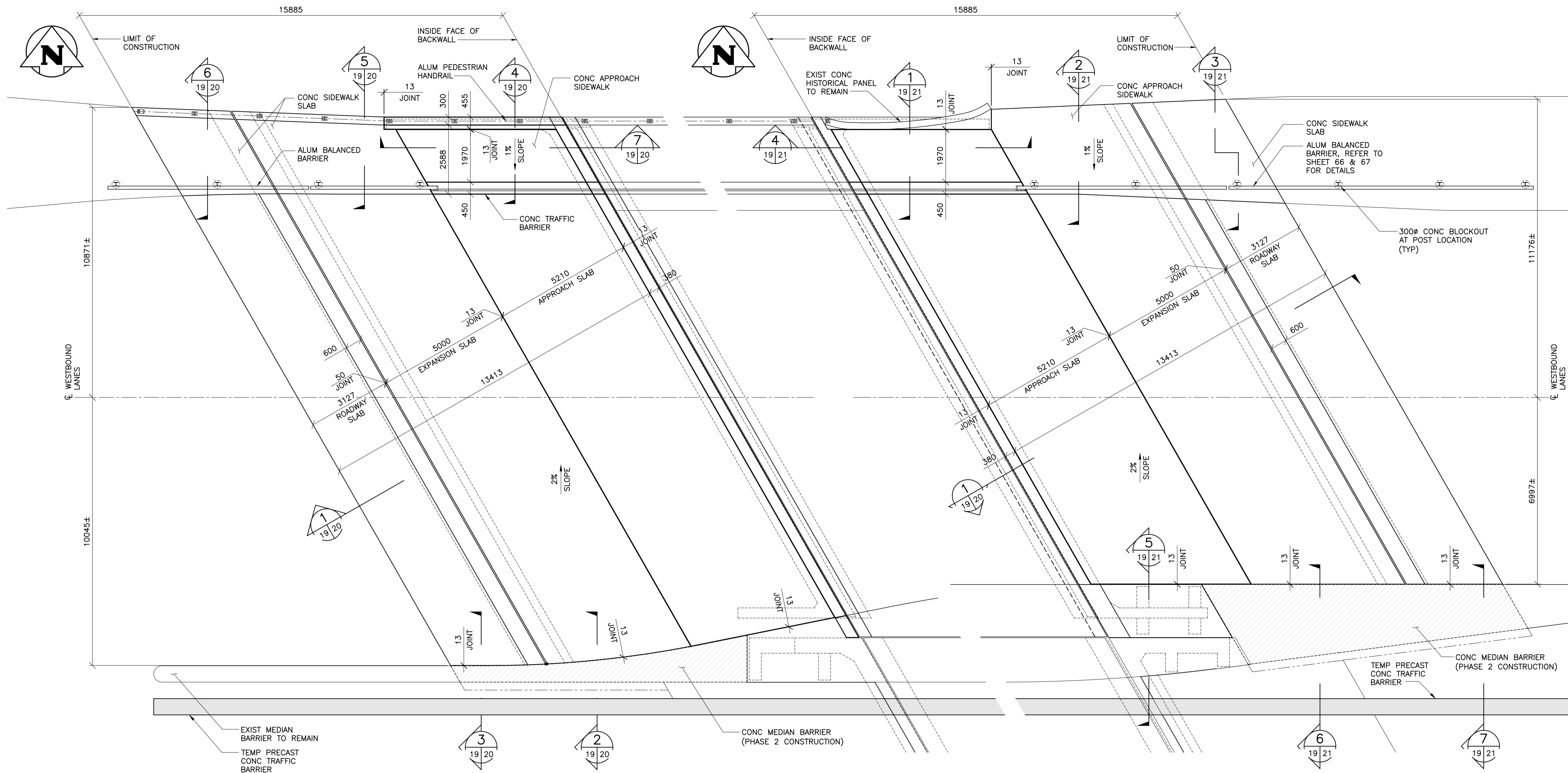
1 WEST APPROACH SLAB - PHASE 1 CONSTRUCTION 1 : 75
