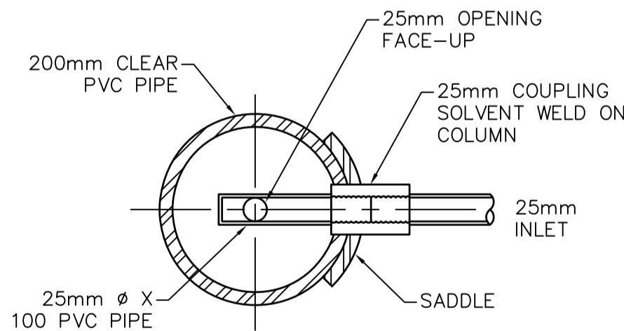
3 DETAIL NTS
