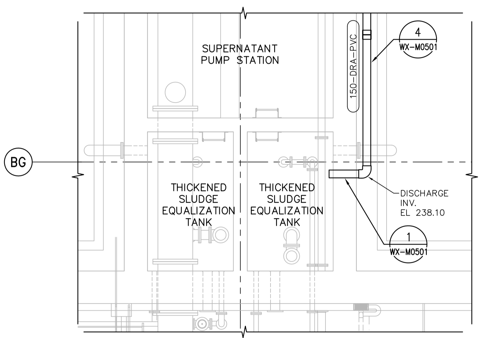
3 PARTIAL PLAN 1:50
