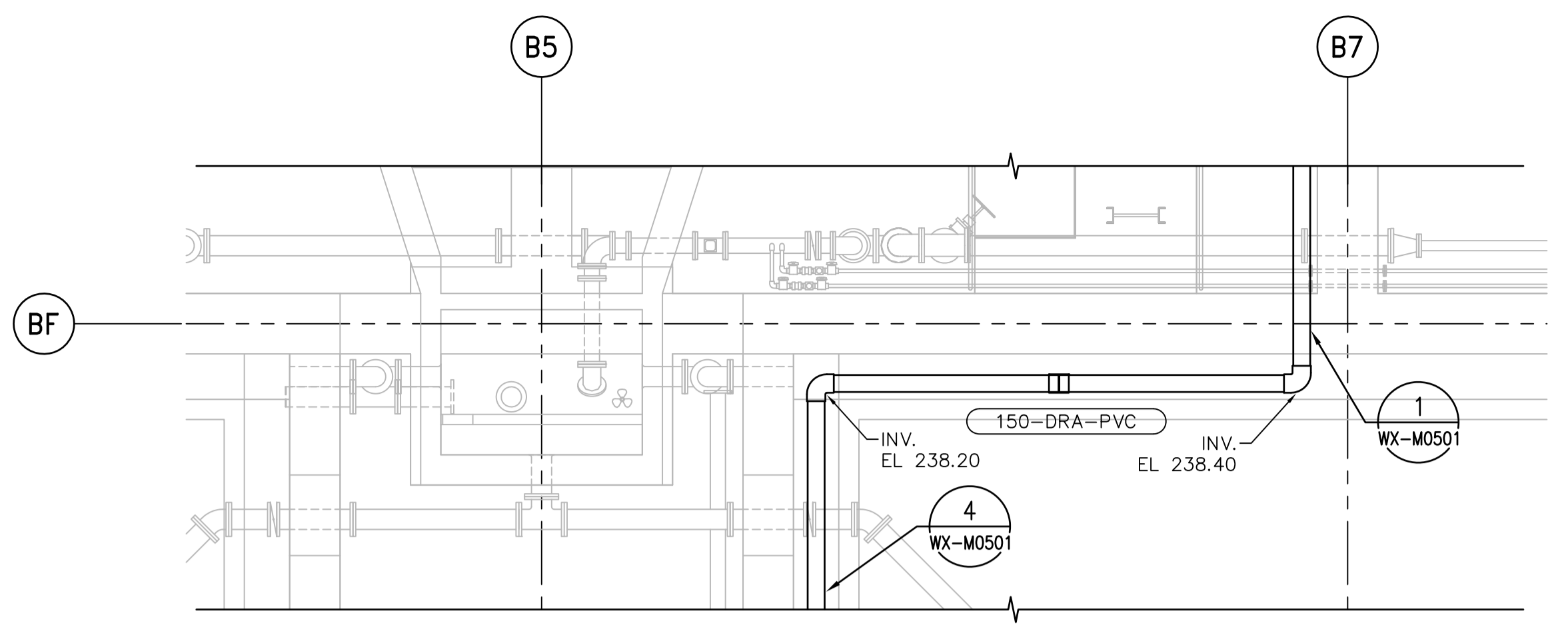
2 PARTIAL PLAN 1:50
