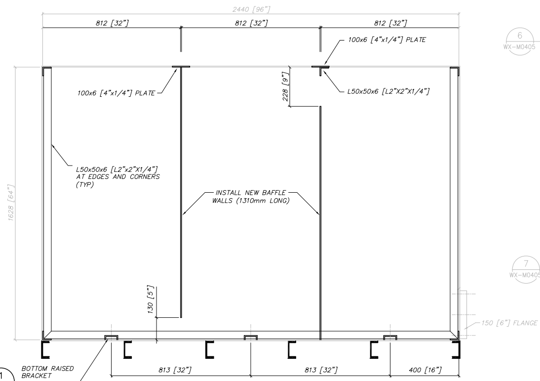
D SECTION 1:10
