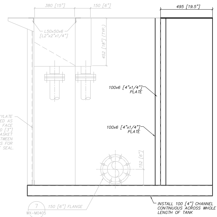
E SECTION 1:10
