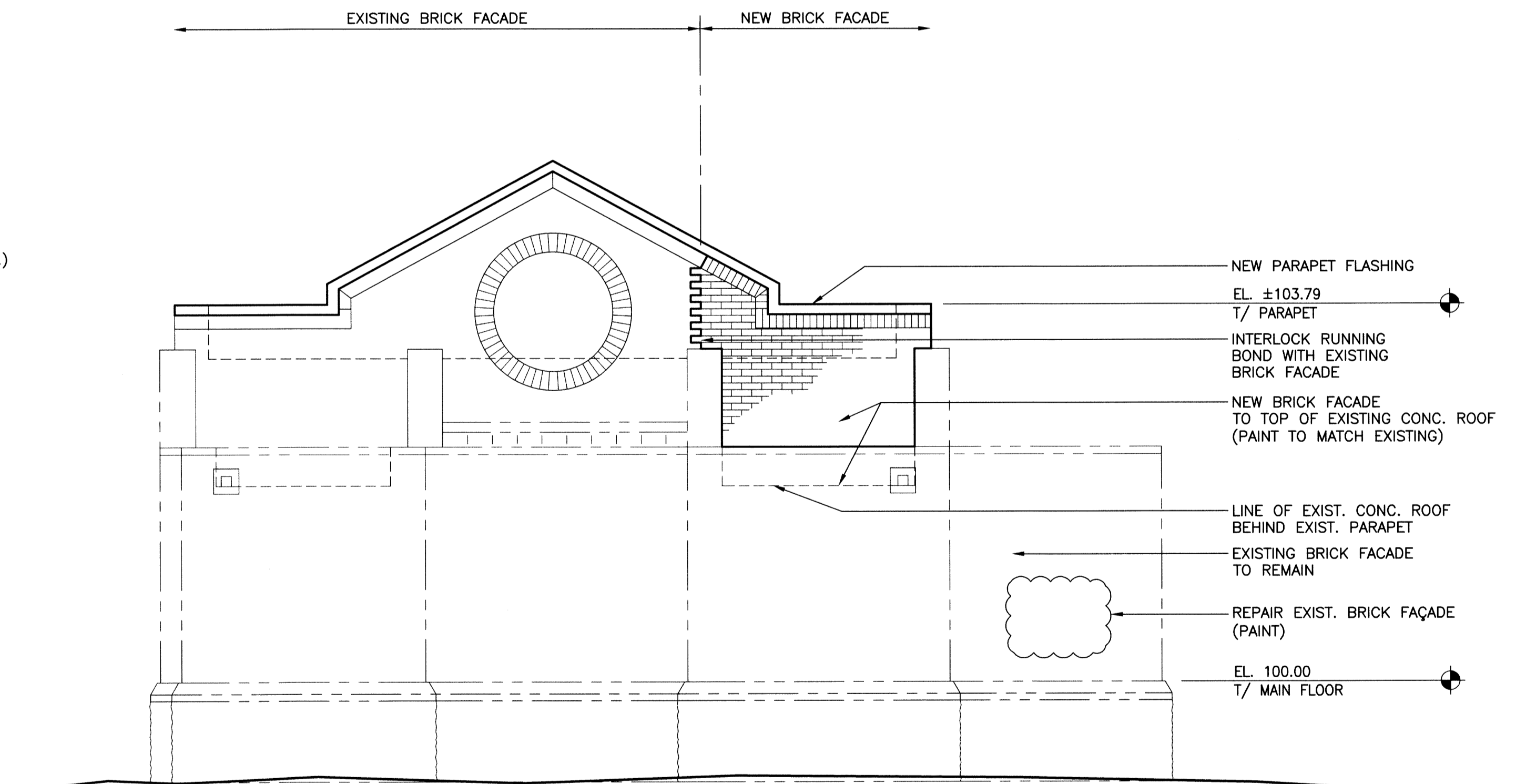
WEST ELEVATION
