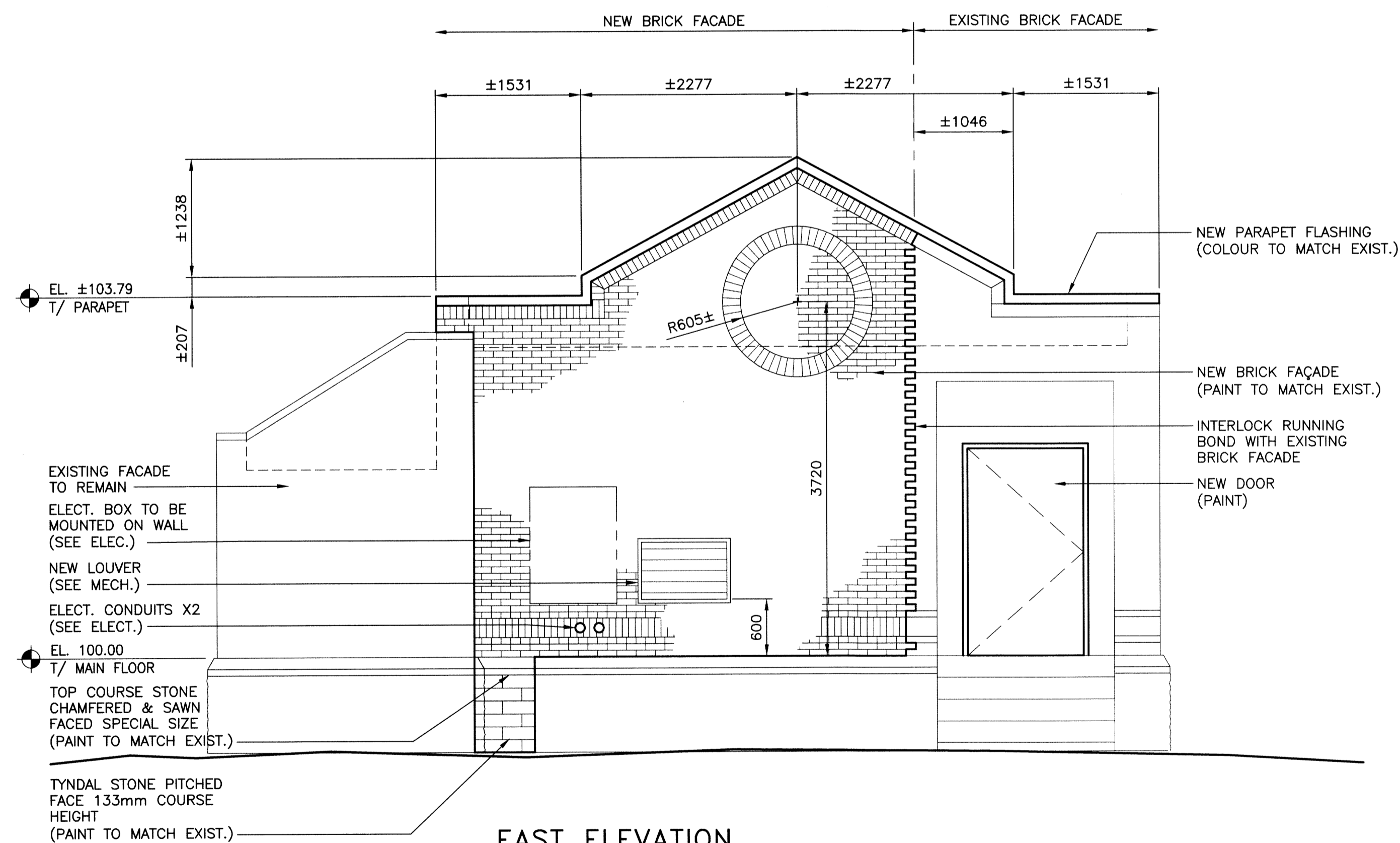
EAST ELEVATION
