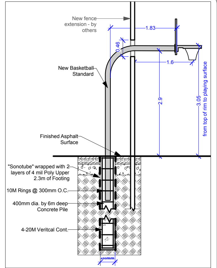
BASKETBALL STANDARD DETAIL - NTS
