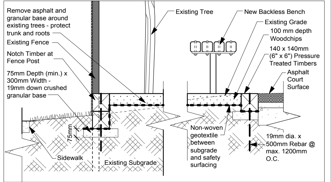
TIMBER EDGING FOR TREE BED DETAIL - NTS
