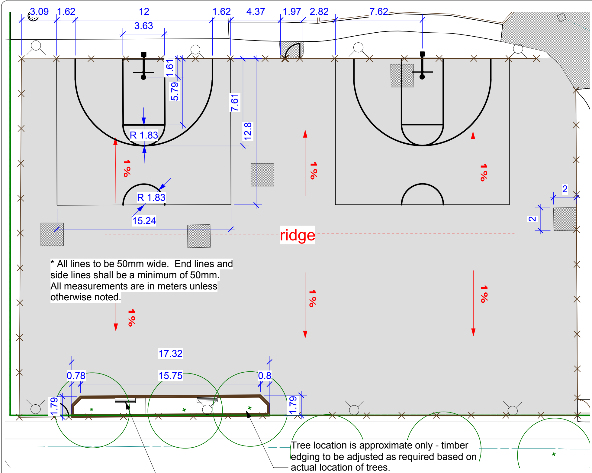
Plan of Timber Edging along Fence
