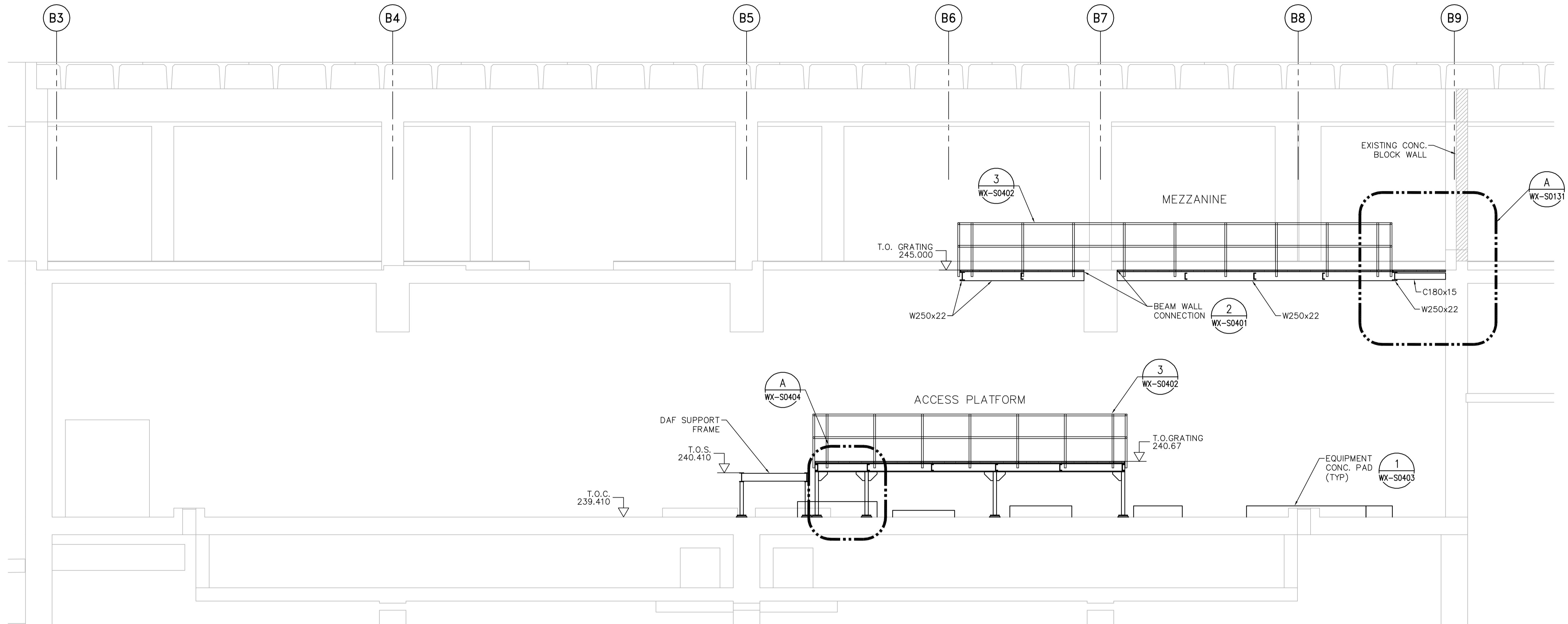
A SECTION 1:50
