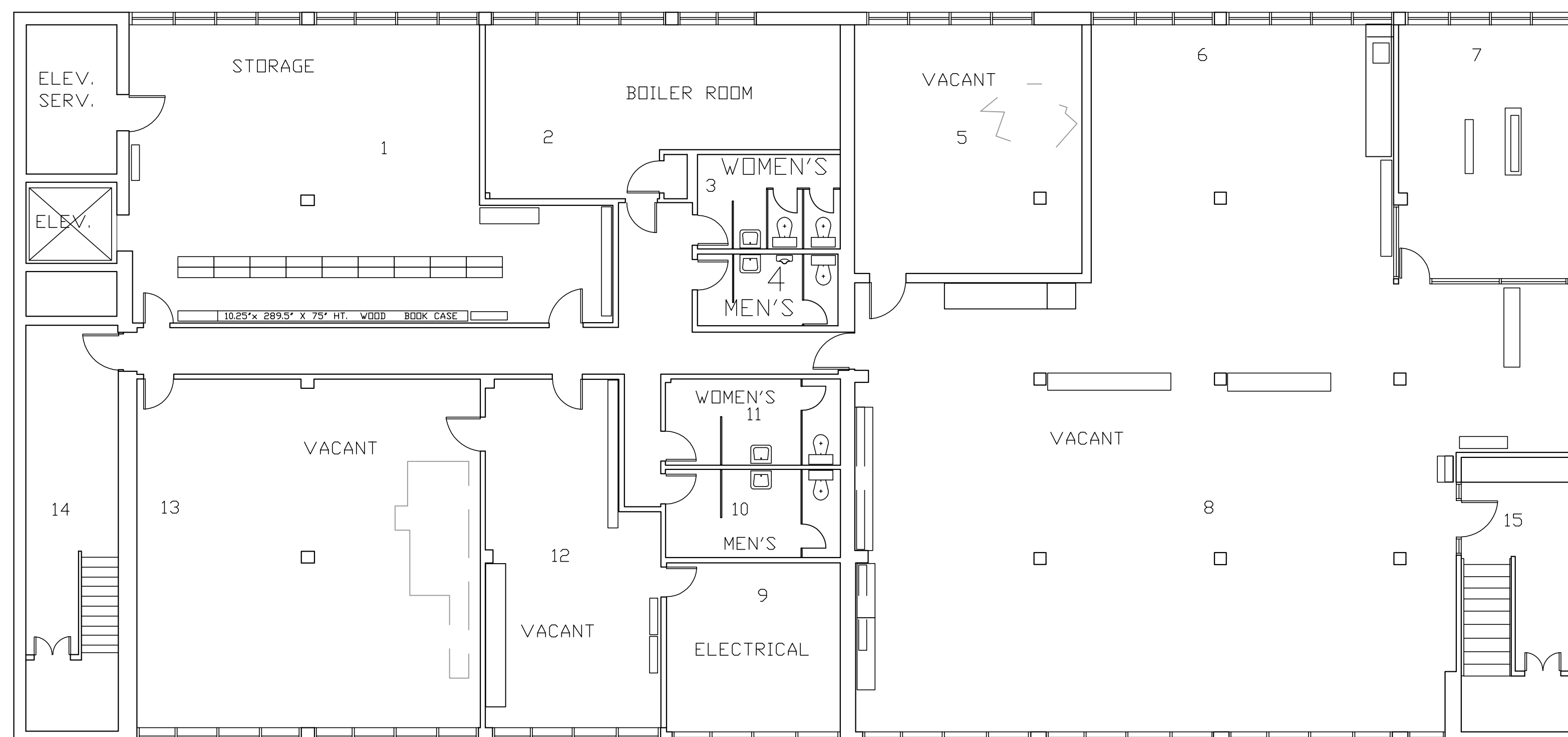
BASEMENT PLAN FOR ELECTRICAL REFERENCE ONLY SCALE 1/8"=1'-0"
