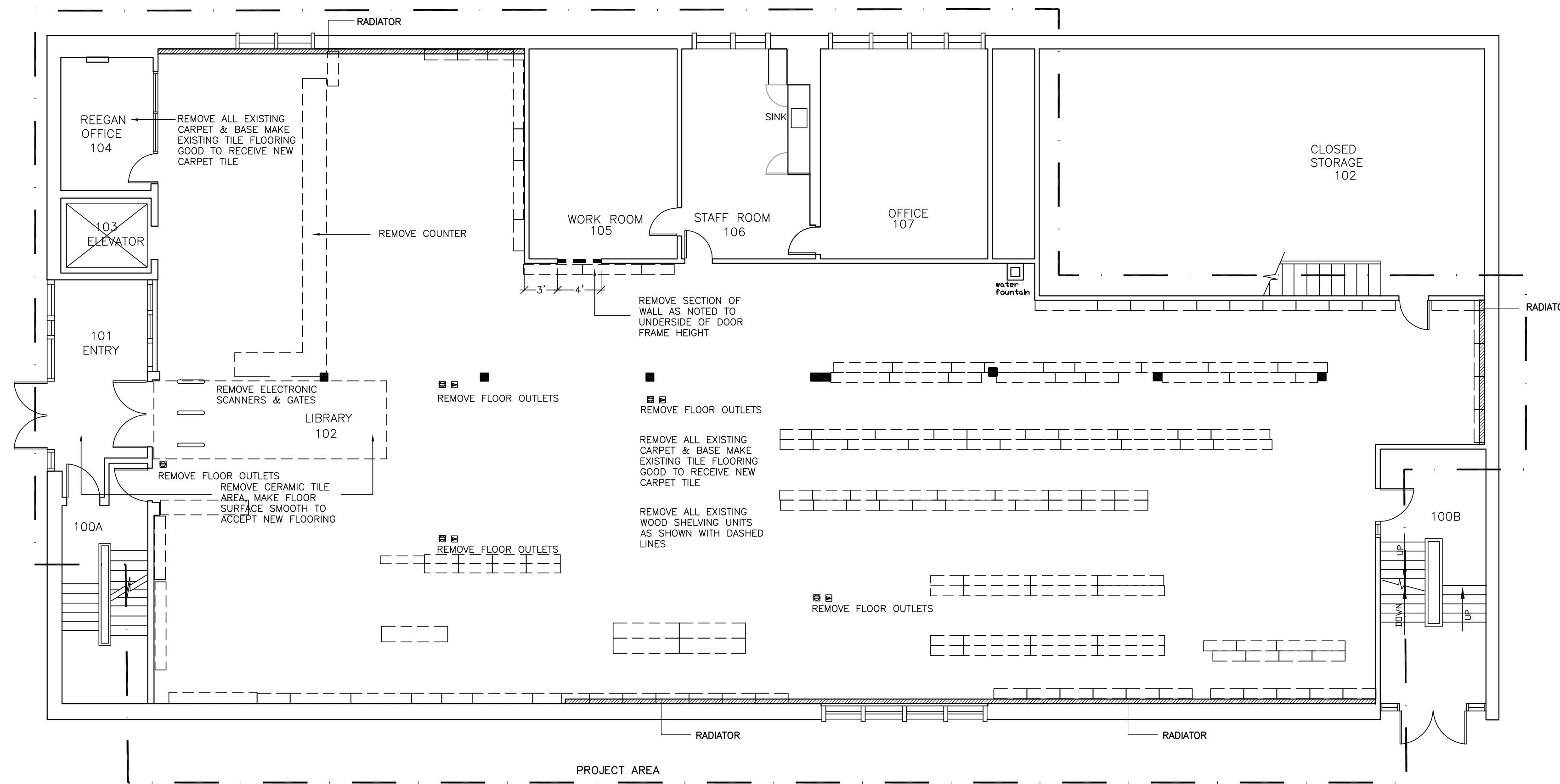
DEMOLITION PLAN SCALE 1/8"=1'-0"
