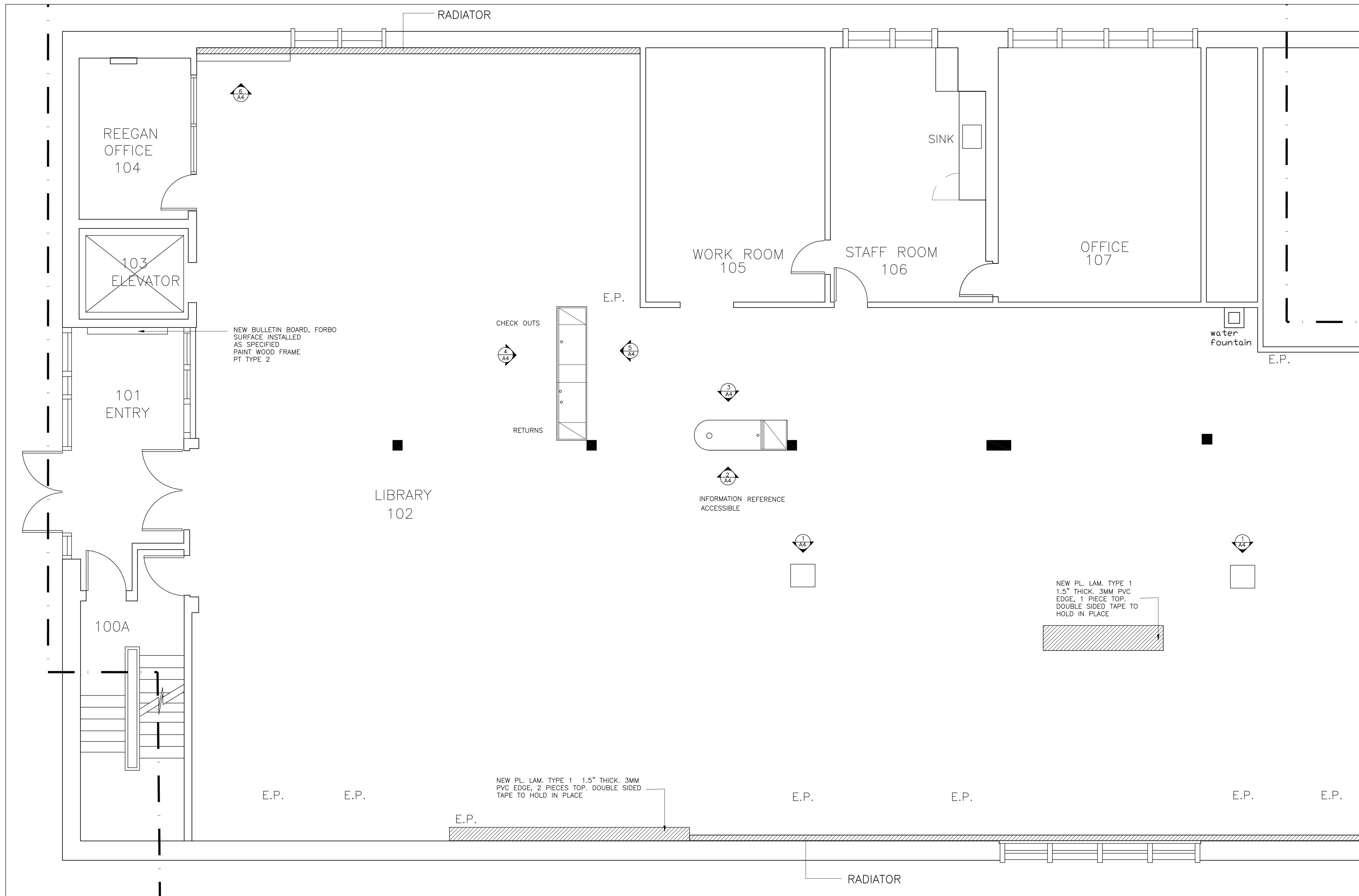
MILLWORK PLAN SCALE 1/4"=1'-0"
