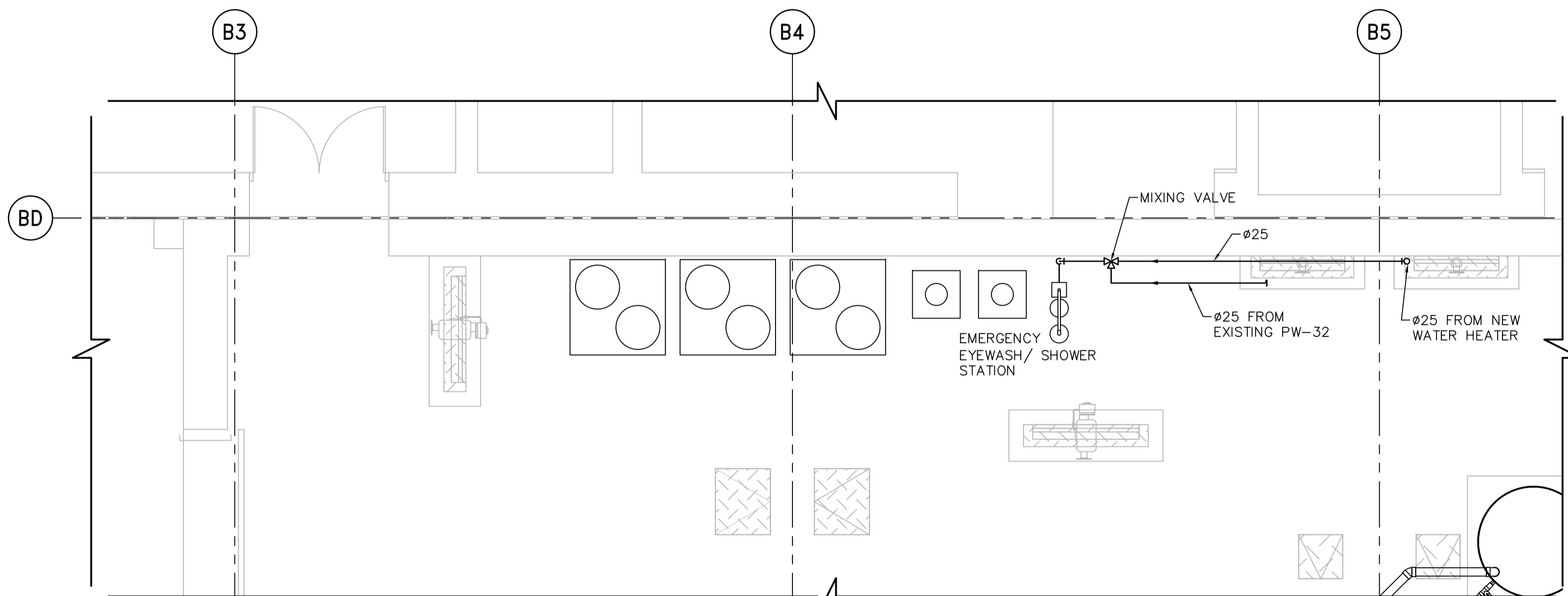
2 PARTIAL PLAN AT 239.410 1:50
