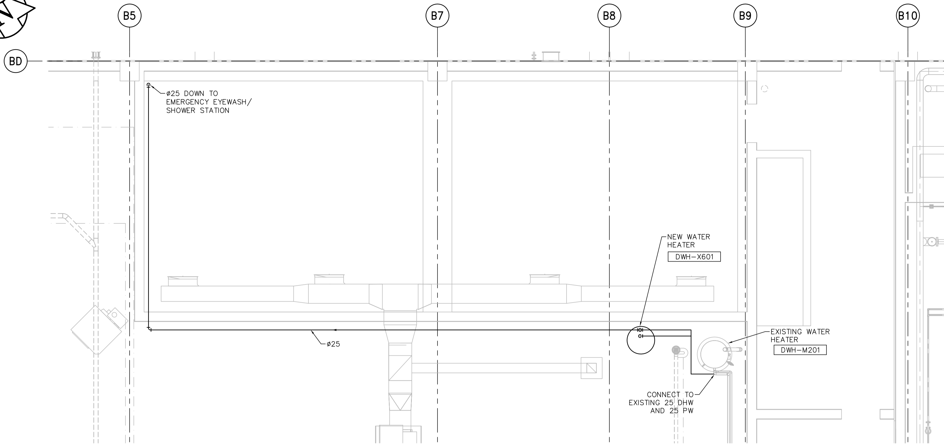
1 PARTIAL PLAN AT 245.00 1:50
