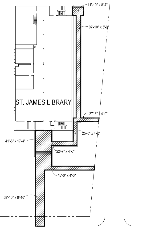
SITE PLAN - SNOW REMOVAL NOT TO SCALE-FOR INFORMATION ONLY
