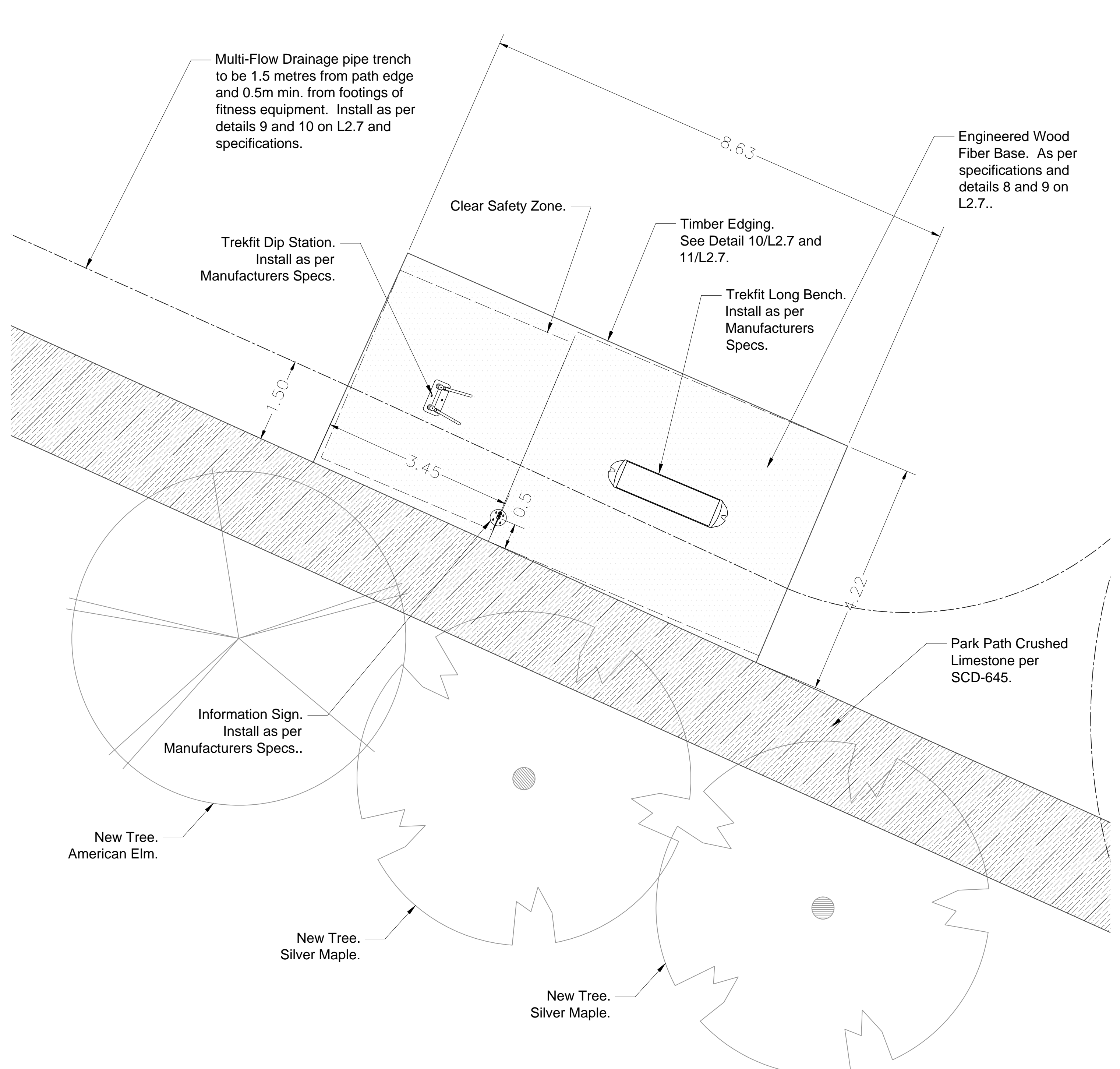
4 FITNESS NODE 4 L2.5 Scale = 1:50
