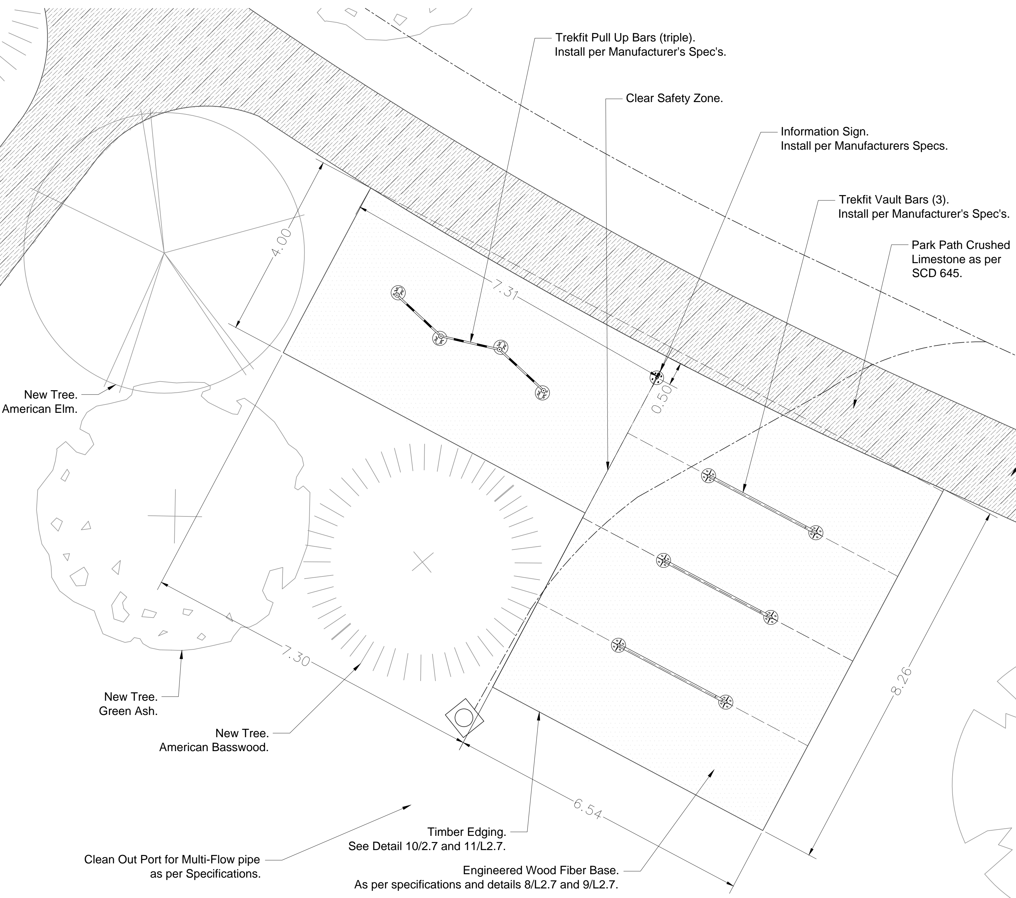
3 FITNESS NODE 3 L2.5 Scale = 1:50
