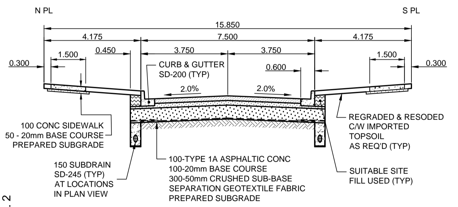
PAVEMENT SECTION ASPHALT PAVEMENT STRUCTURE TYPICAL SCALE: N.T.S.
