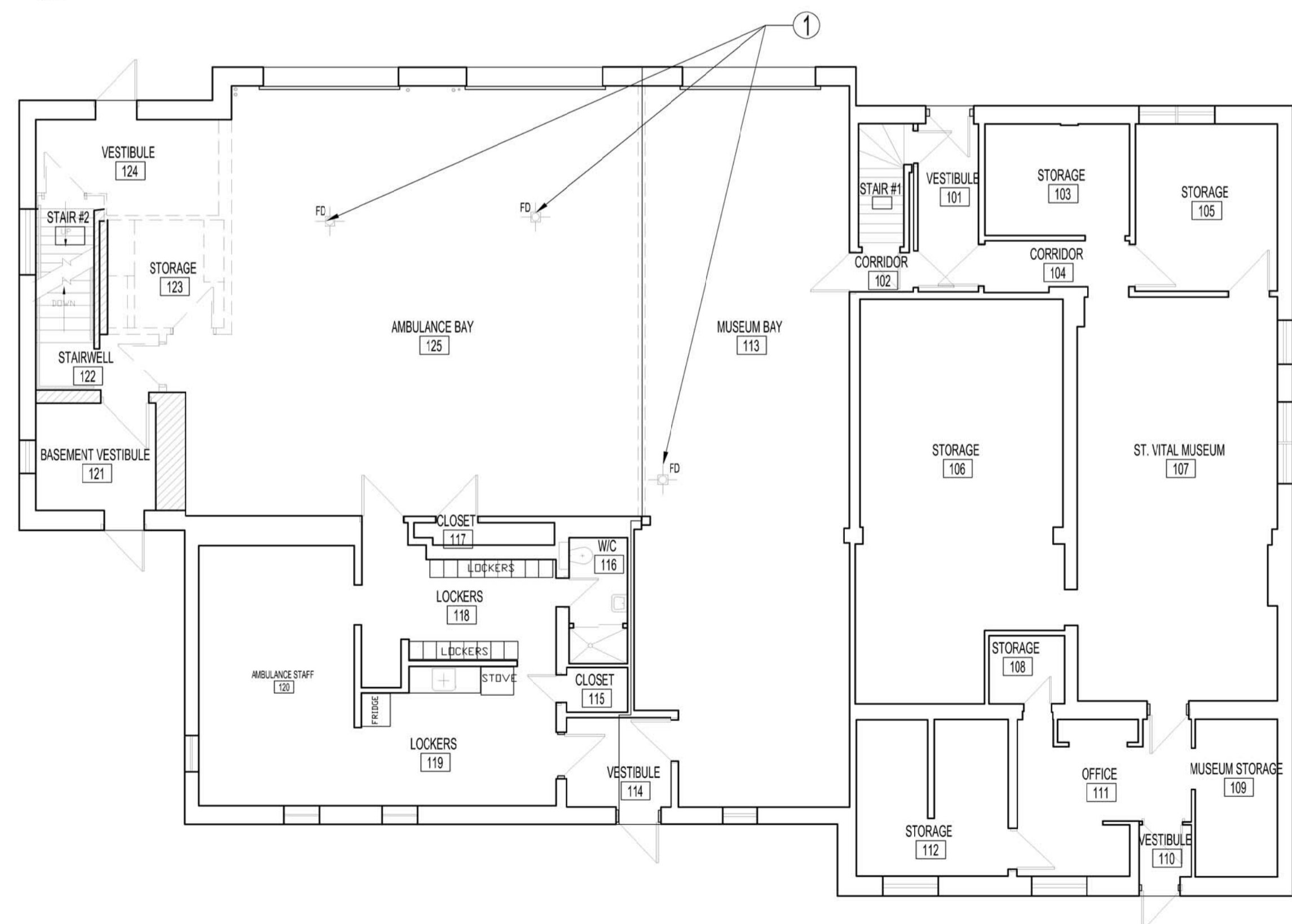
2 MAIN FLOOR PLAN - PLUMBING DEMOLITION M3 M3 SCALE: 1/8"=1'-0"
