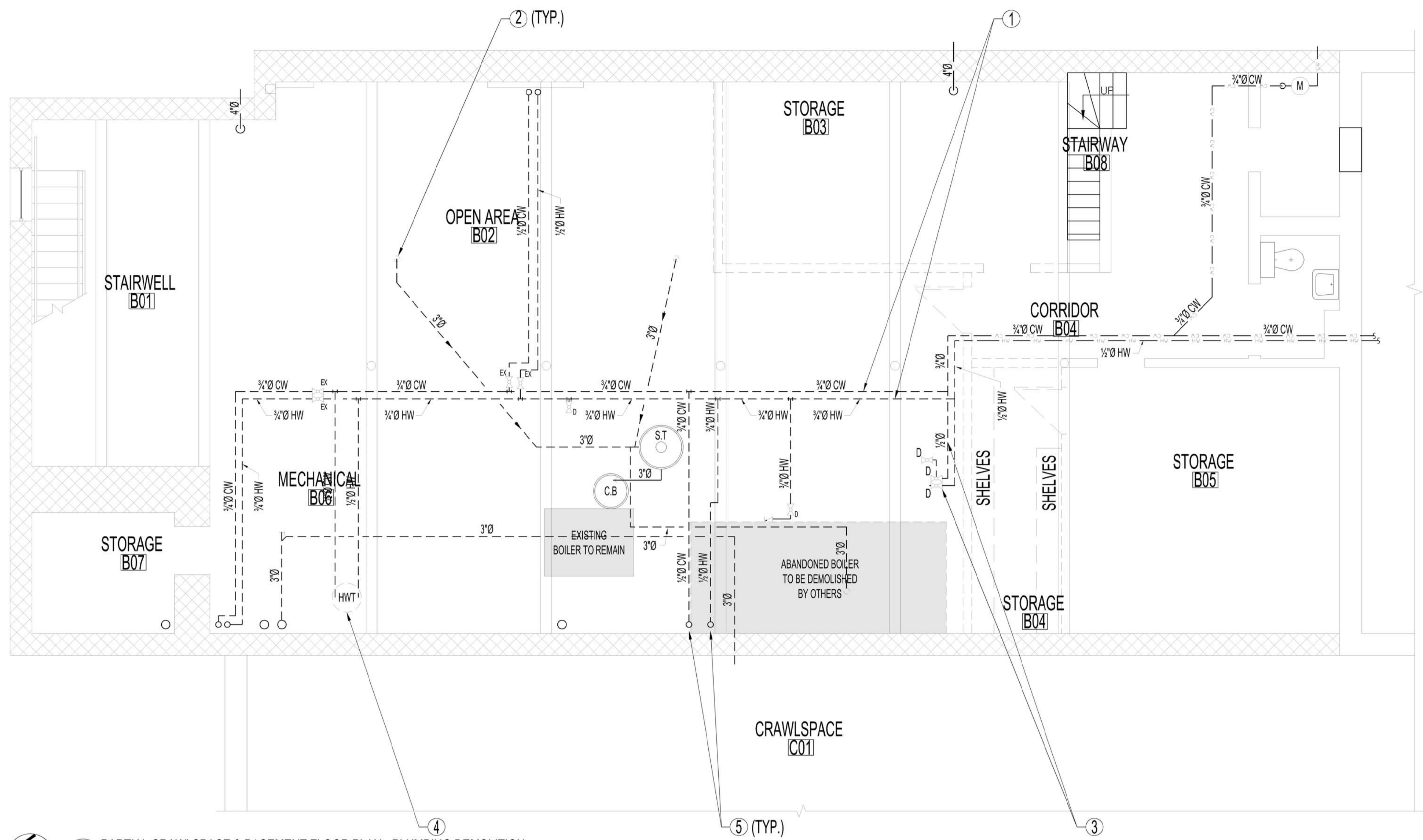
1 PARTIAL CRAWLSPACE & BASEMENT FLOOR PLAN - PLUMBING DEMOLITION M3 M3 SCALE: 1/4"=1'-0"
