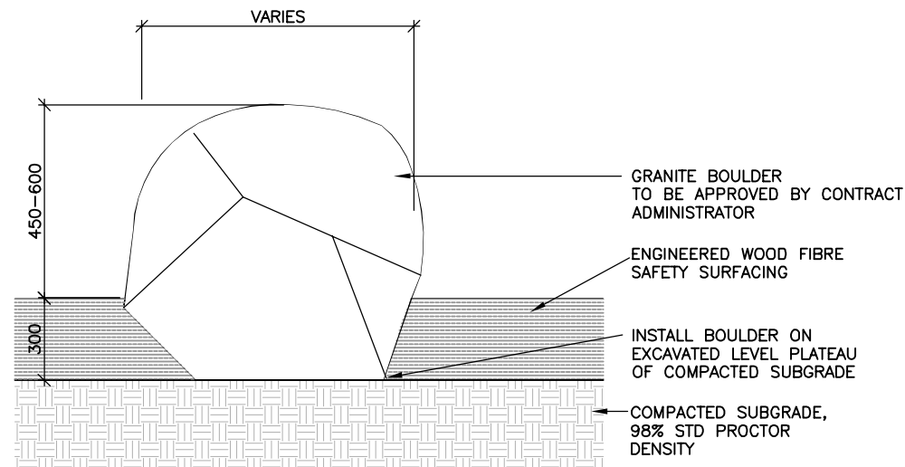
3 GRANITE BOULDER L1-2 | L1-3 1:25
