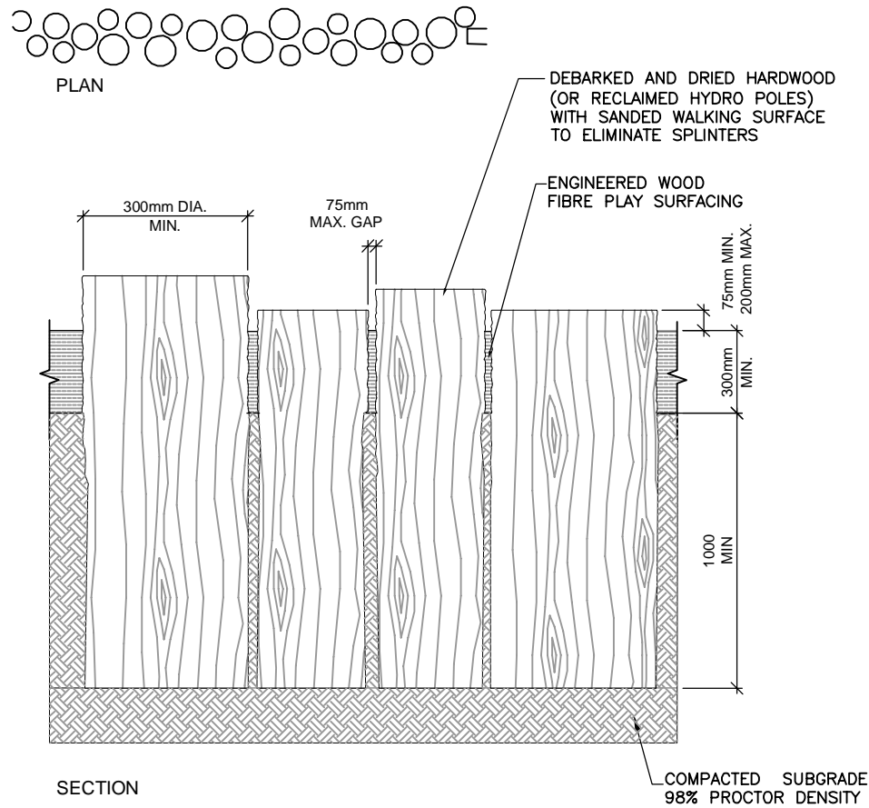
2 DRIED HARDWOOD STEP POST/EDGING L1-2 | L1-3 1:25
