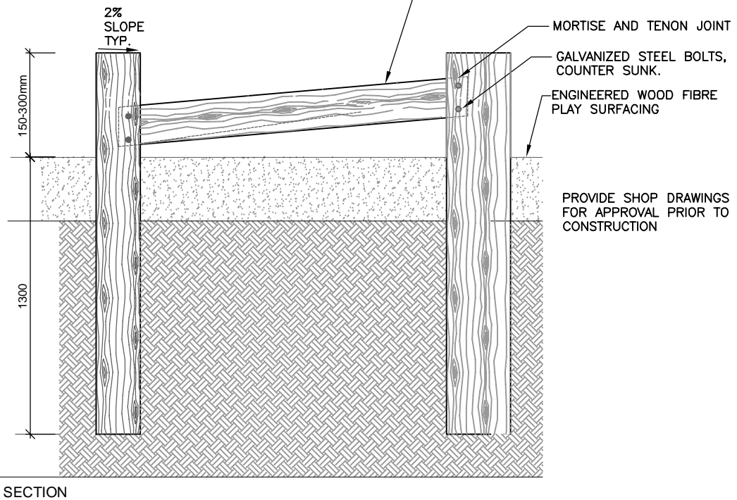
1 DRIED HARDWOOD BALANCE BEAM L1-2 | L1-3 1:25
