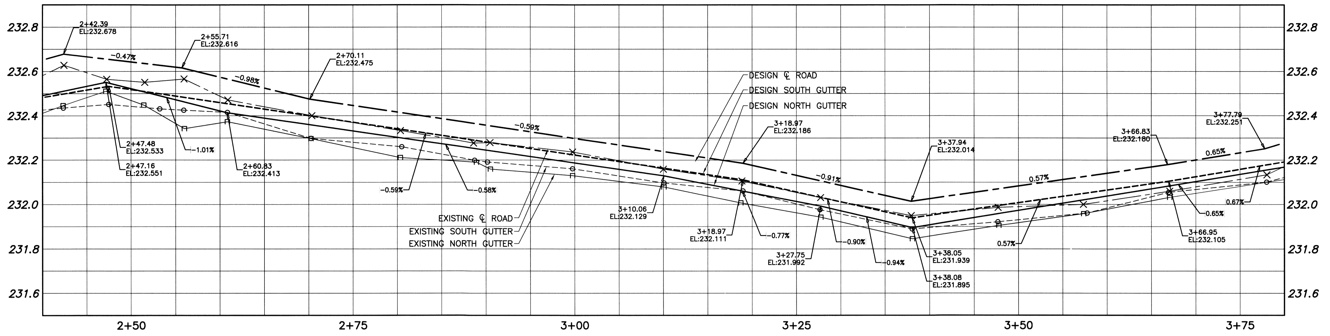
PROFILE SCALE H=1:250 V=1:10
