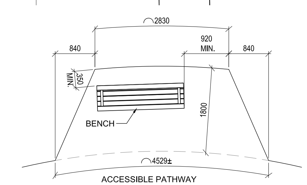
2 TYPICAL SEATING LAYOUT SCALE - 1 : 50
