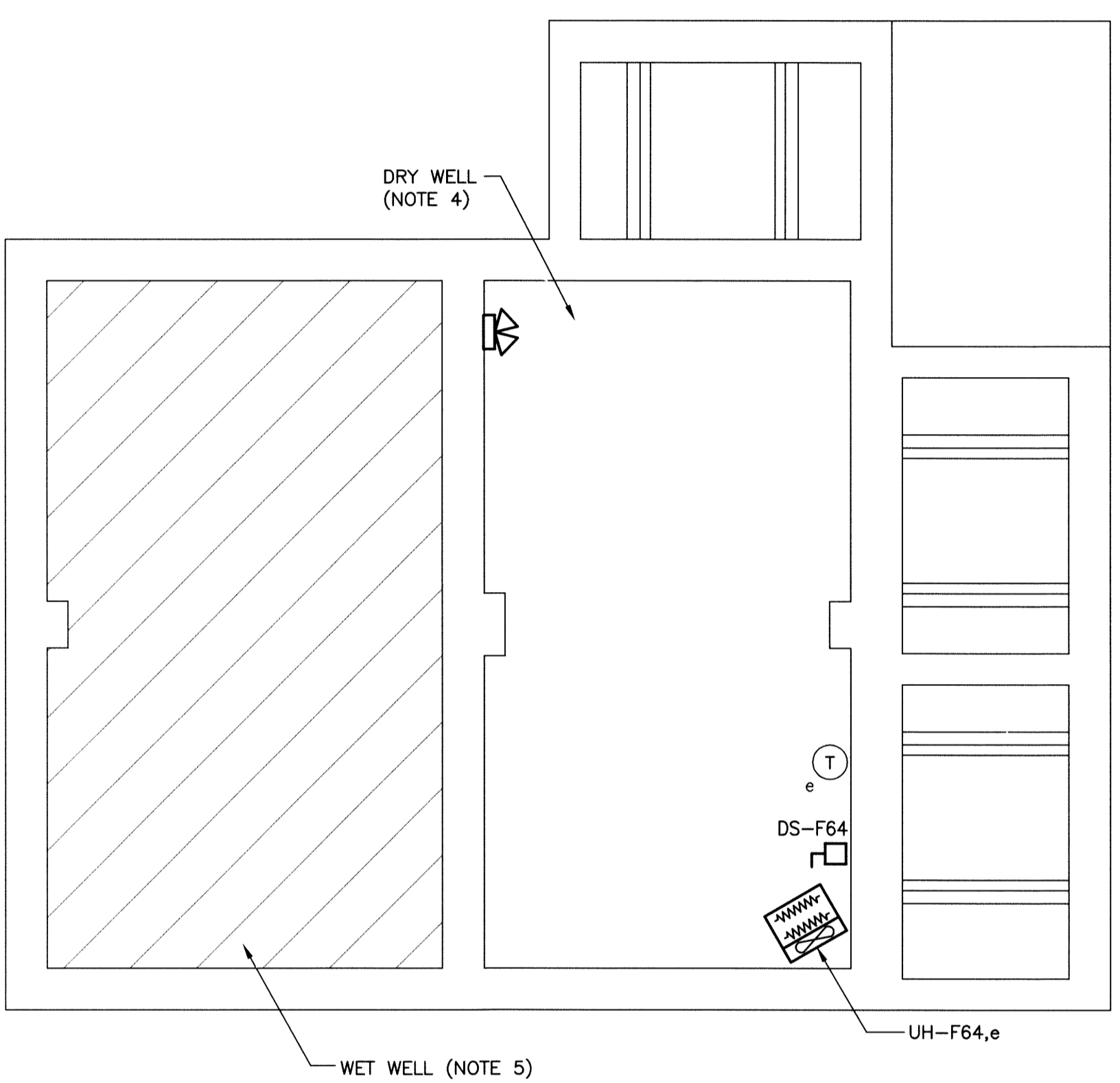
2 LOWER LEVEL PLAN - NEW SCALE: 1:50mm
