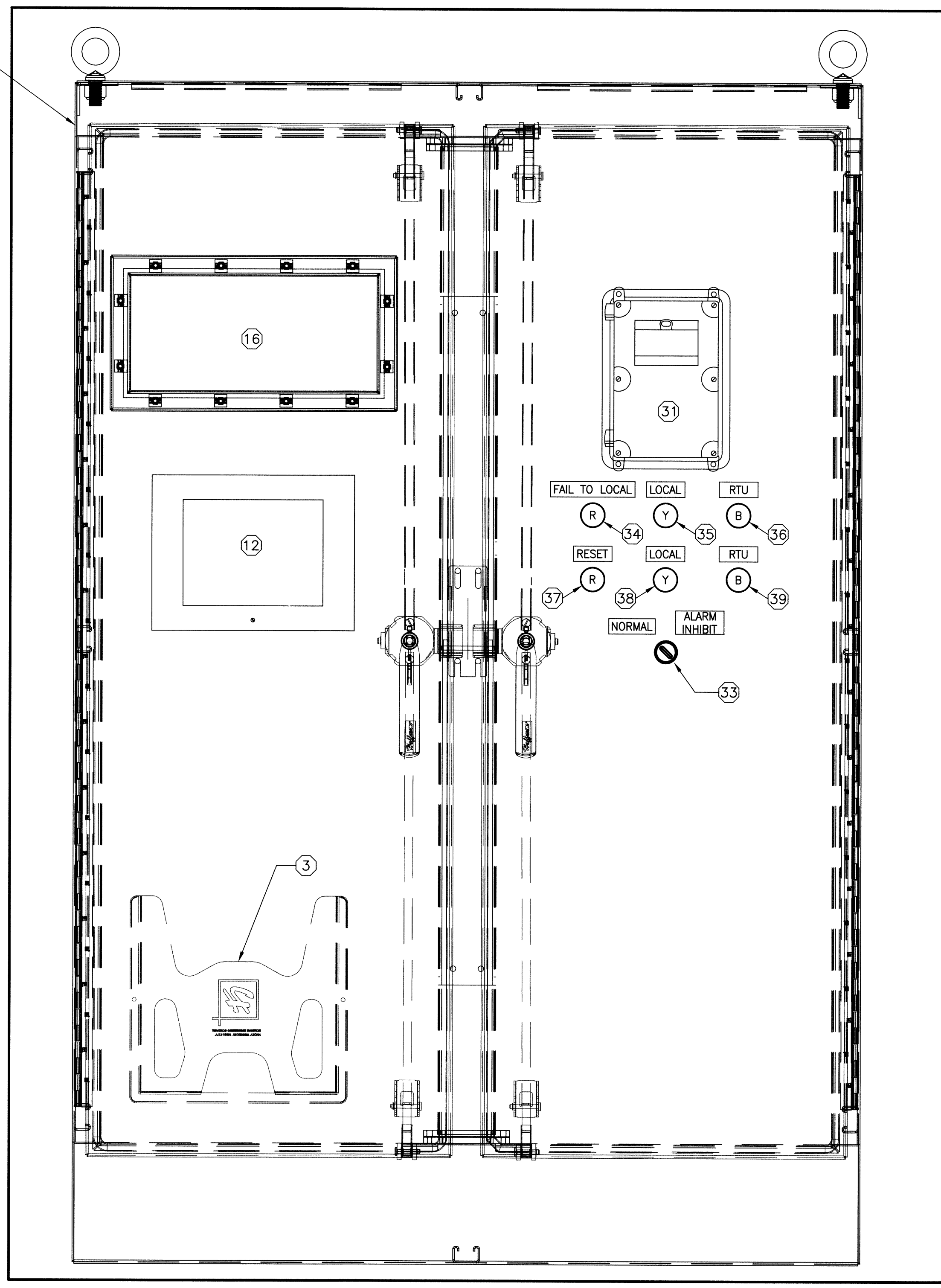
2 ENCLOSURE AND DEVICE FRONT PANEL SCALE: N.T.S.
