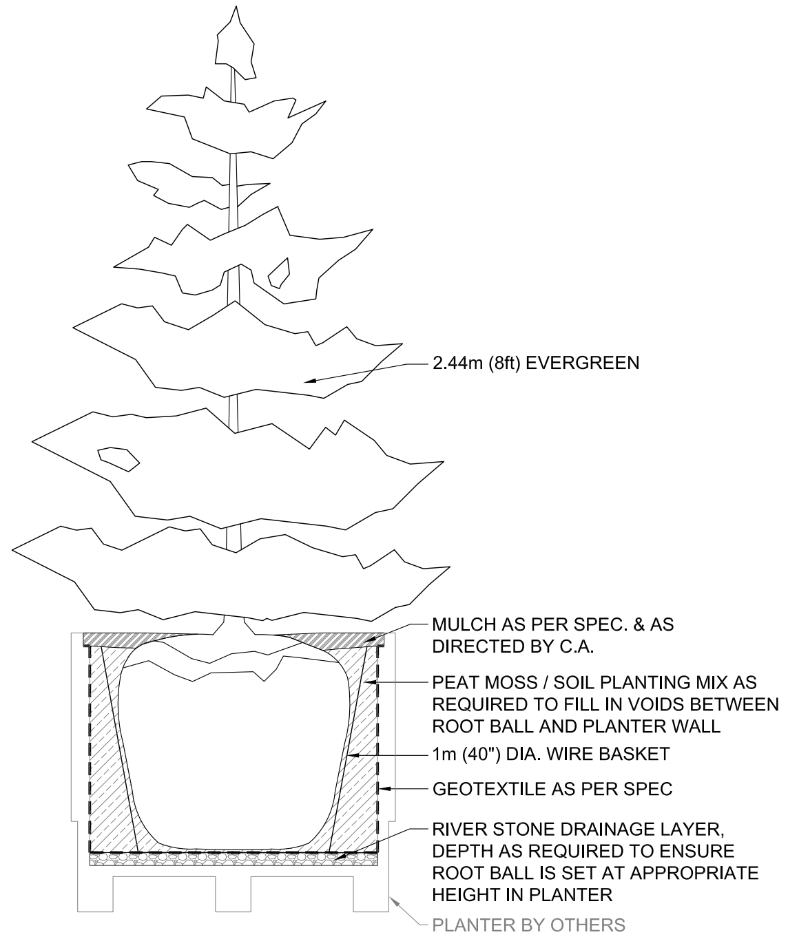
1 TYPICAL TREE PLANTING L101 SCALE - 1 : 20
