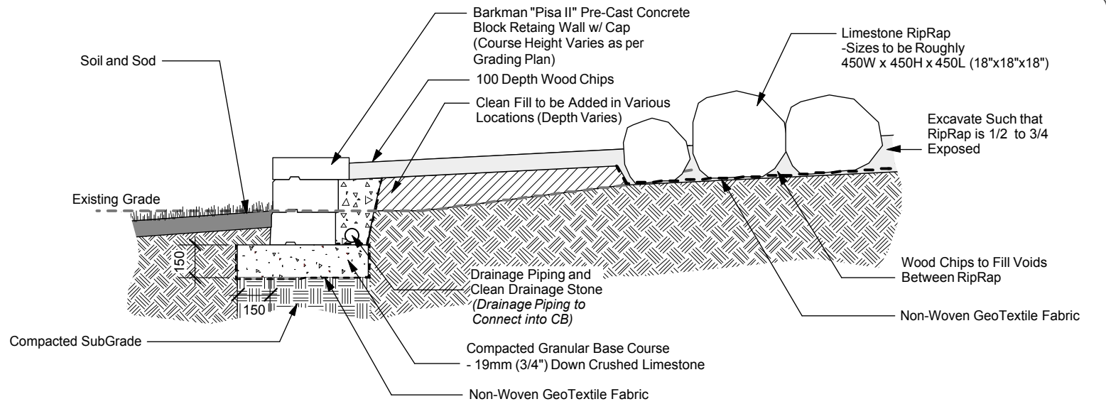
1 Pre-Cast Concrete Block Wall and RipRap Detail 1:25
