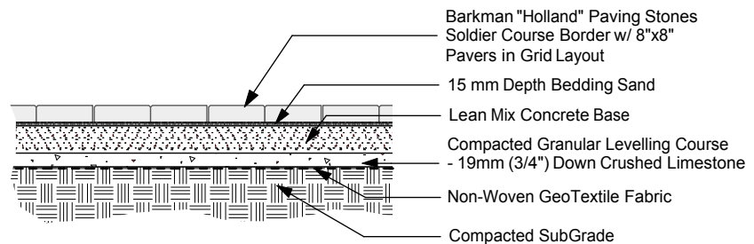
2 Paving Stone on Lean-Mix Concrete Base 1:25
